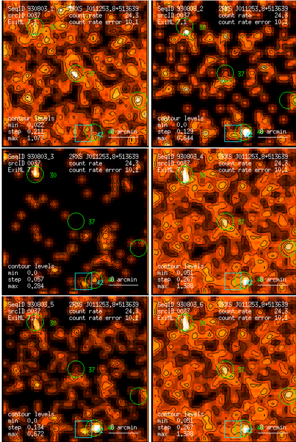
Figure 37: RASS 930803: detection 0037: band rate images, Gaussian filter: (1) PSPC channels 11 – 41, (2) 52 – 90, (3) 91 – 201, (4) 11 – 235, (5) 52 – 201, (6) 11 – 201. Broad band rates in counts/ks. Band rate contour levels in counts/ks/arcmin 2 .
