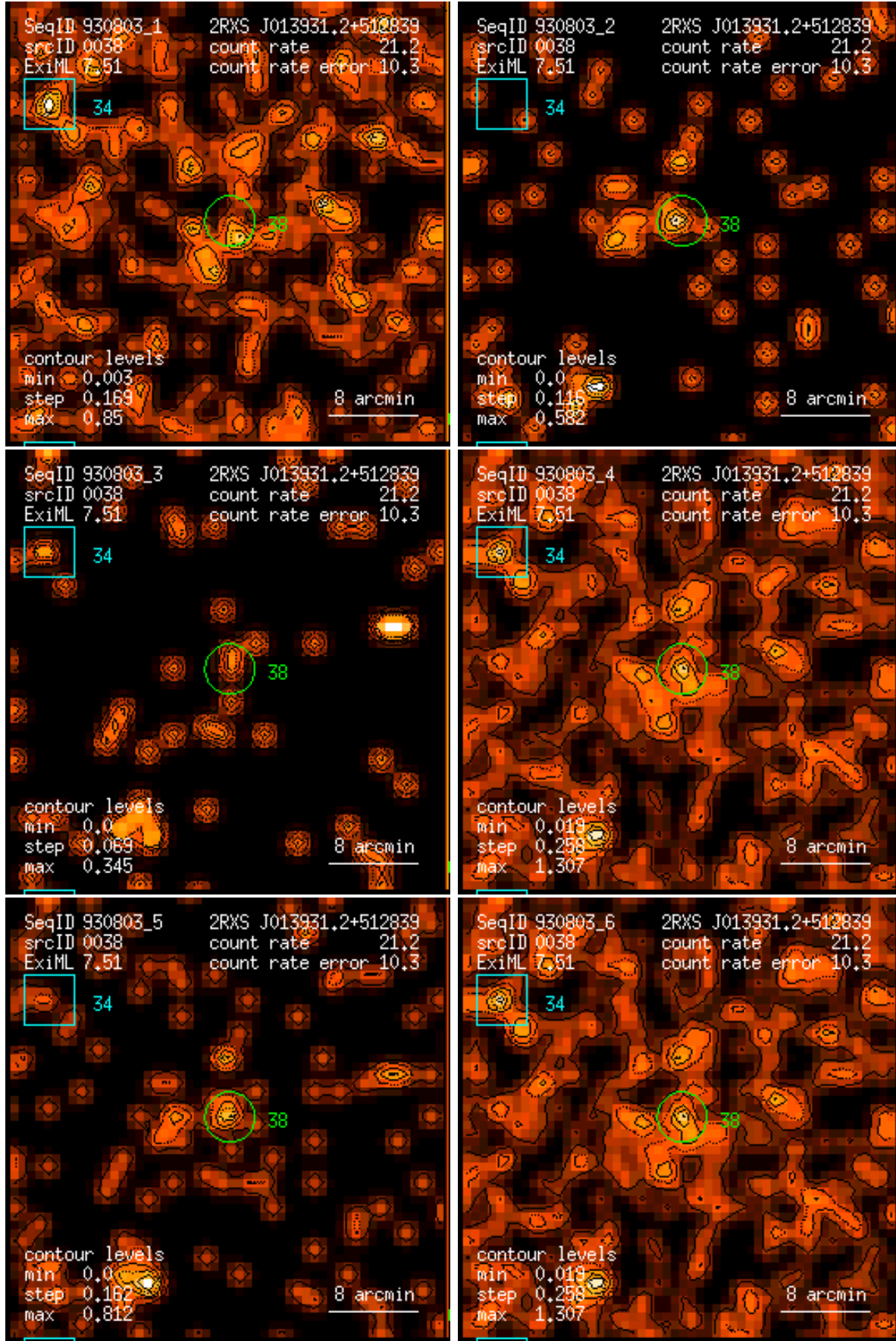
Figure 38: RASS 930803: detection 0038: band rate images, Gaussian filter: (1) PSPC channels 11 – 41, (2) 52 – 90, (3) 91 – 201, (4) 11 – 235, (5) 52 – 201, (6) 11 – 201. Broad band rates in counts/ks. Band rate contour levels in counts/ks/arcmin 2 .
