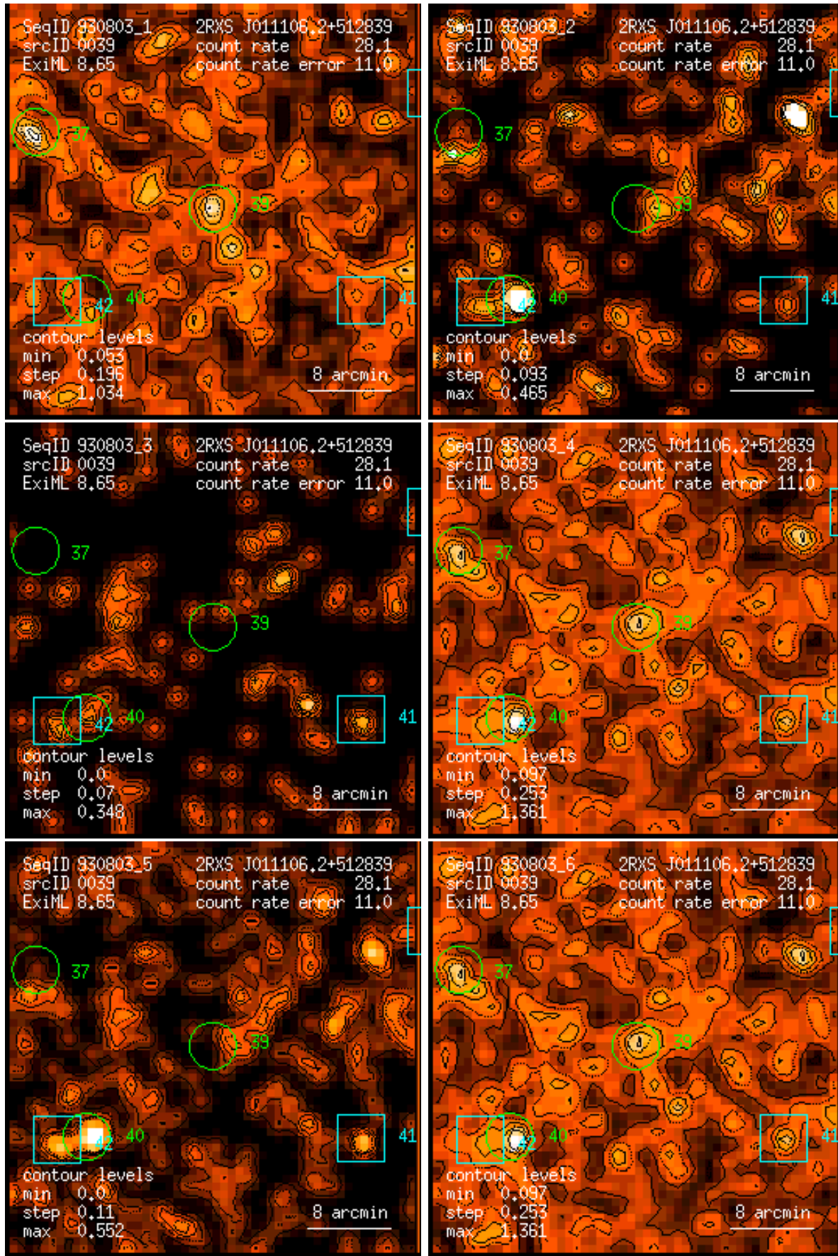
Figure 39: RASS 930803: detection 0039: band rate images, Gaussian filter: (1) PSPC channels 11 – 41, (2) 52 – 90, (3) 91 – 201, (4) 11 – 235, (5) 52 – 201, (6) 11 – 201. Broad band rates in counts/ks. Band rate contour levels in counts/ks/arcmin 2 .
