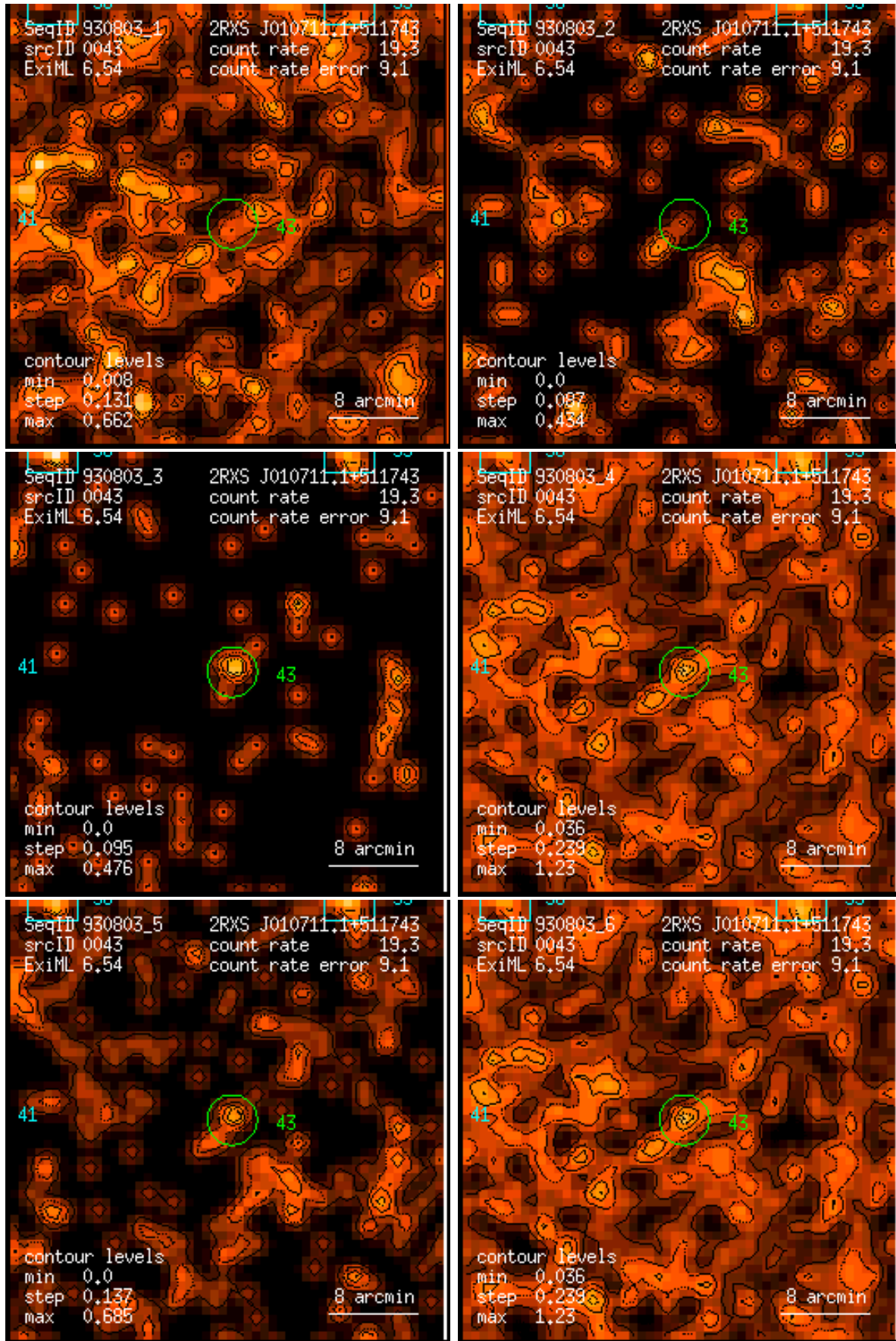
Figure 43: RASS 930803: detection 0043: band rate images, Gaussian filter: (1) PSPC channels 11 – 41, (2) 52 – 90, (3) 91 – 201, (4) 11 – 235, (5) 52 – 201, (6) 11 – 201. Broad band rates in counts/ks. Band rate contour levels in counts/ks/arcmin 2 .
