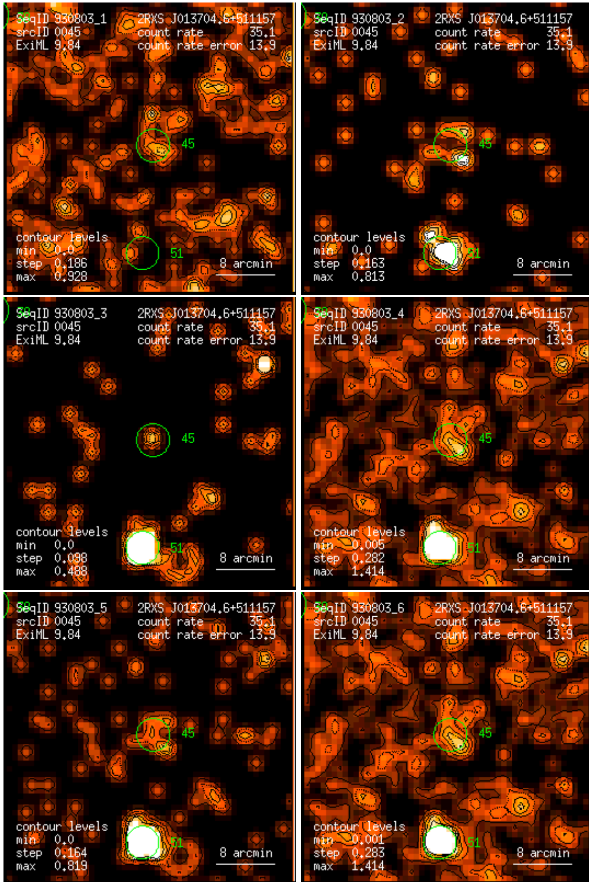
Figure 45: RASS 930803: detection 0045: band rate images, Gaussian filter: (1) PSPC channels 11 – 41, (2) 52 – 90, (3) 91 – 201, (4) 11 – 235, (5) 52 – 201, (6) 11 – 201. Broad band rates in counts/ks. Band rate contour levels in counts/ks/arcmin 2 .
