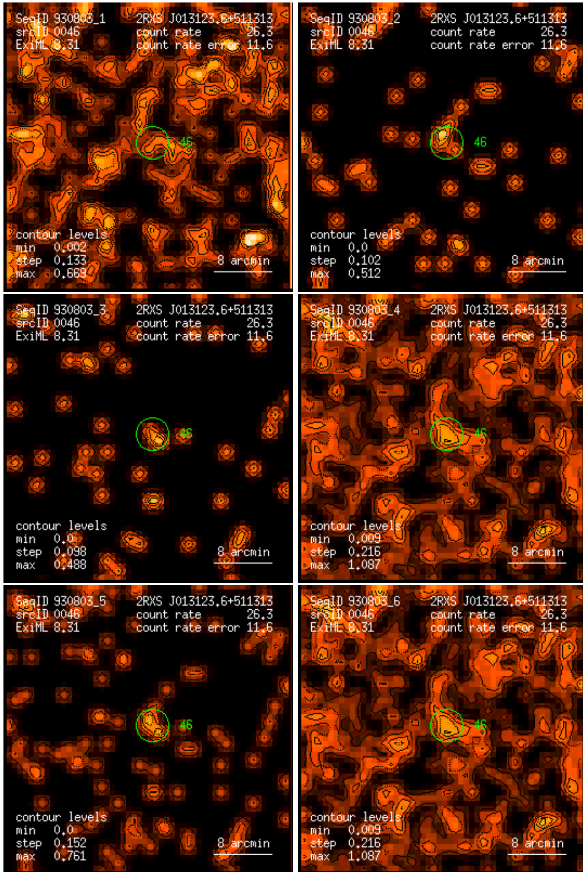
Figure 46: RASS 930803: detection 0046: band rate images, Gaussian filter: (1) PSPC channels 11 – 41, (2) 52 – 90, (3) 91 – 201, (4) 11 – 235, (5) 52 – 201, (6) 11 – 201. Broad band rates in counts/ks. Band rate contour levels in counts/ks/arcmin 2 .
