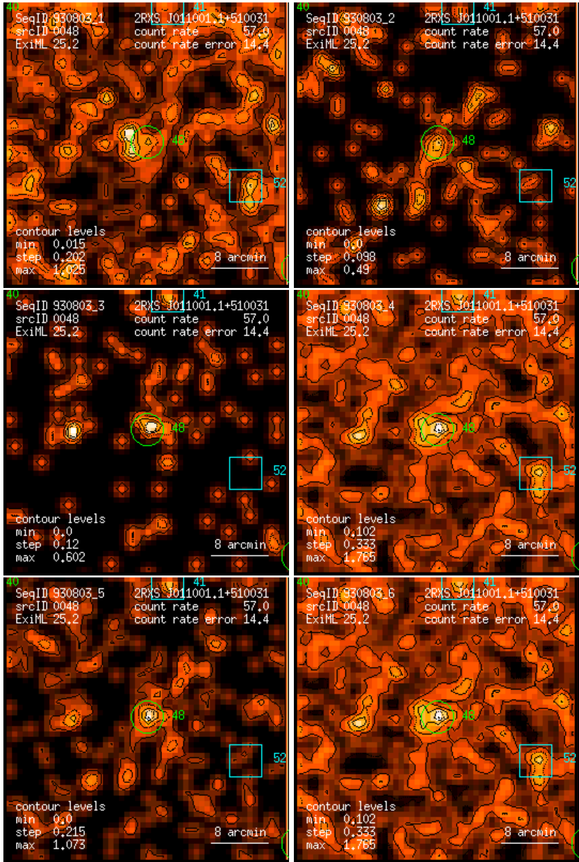
Figure 48: RASS 930803: detection 0048: band rate images, Gaussian filter: (1) PSPC channels 11 – 41, (2) 52 – 90, (3) 91 – 201, (4) 11 – 235, (5) 52 – 201, (6) 11 – 201. Broad band rates in counts/ks. Band rate contour levels in counts/ks/arcmin 2 .
