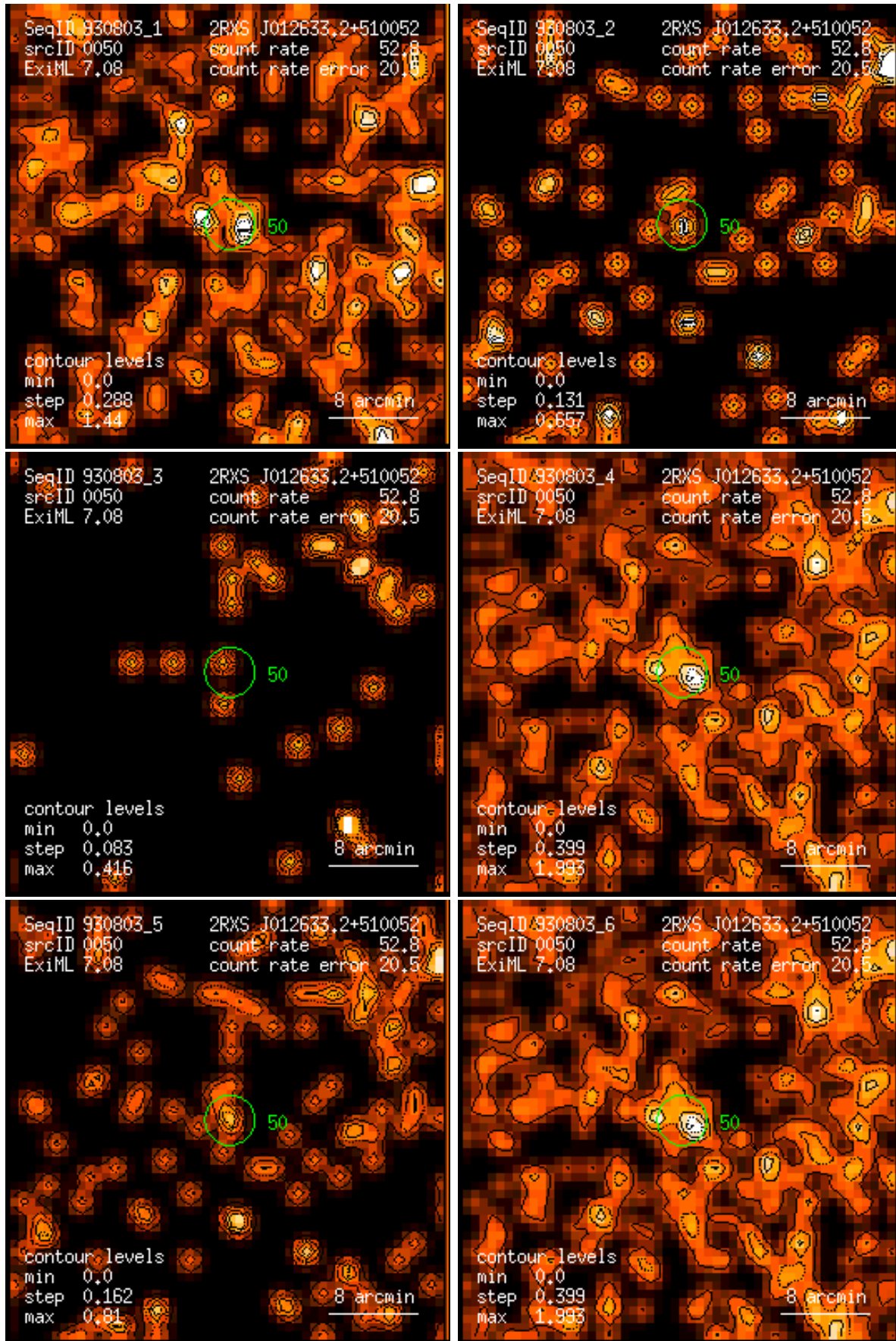
Figure 50: RASS 930803: detection 0050: band rate images, Gaussian filter: (1) PSPC channels 11 – 41, (2) 52 – 90, (3) 91 – 201, (4) 11 – 235, (5) 52 – 201, (6) 11 – 201. Broad band rates in counts/ks. Band rate contour levels in counts/ks/arcmin 2 .
