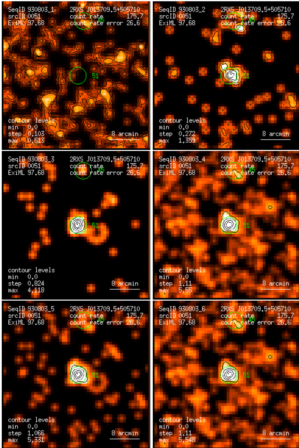
Figure 51: RASS 930803: detection 0051: band rate images, Gaussian filter: (1) PSPC channels 11 – 41, (2) 52 – 90, (3) 91 – 201, (4) 11 – 235, (5) 52 – 201, (6) 11 – 201. Broad band rates in counts/ks. Band rate contour levels in counts/ks/arcmin 2 .
