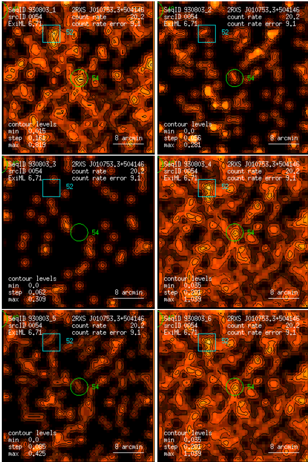
Figure 54: RASS 930803: detection 0054: band rate images, Gaussian filter: (1) PSPC channels 11 – 41, (2) 52 – 90, (3) 91 – 201, (4) 11 – 235, (5) 52 – 201, (6) 11 – 201. Broad band rates in counts/ks. Band rate contour levels in counts/ks/arcmin 2 .
