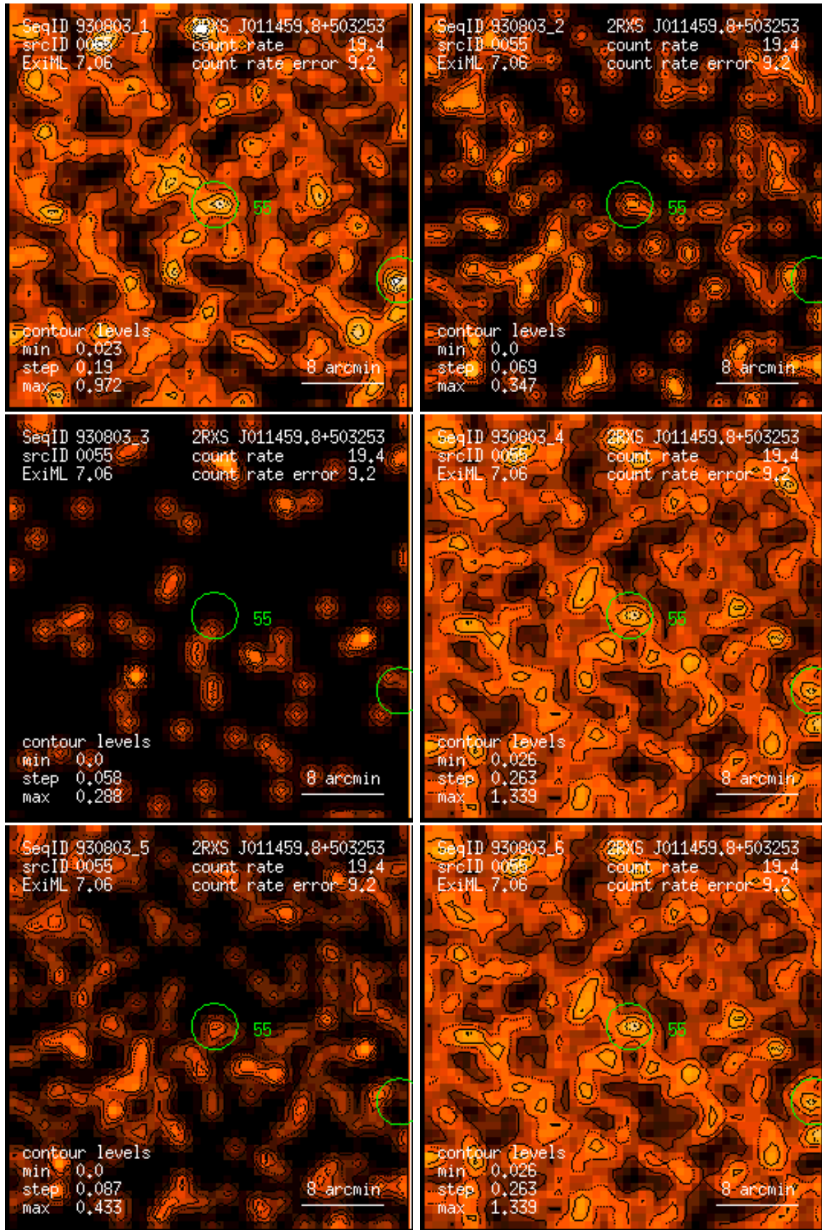
Figure 55: RASS 930803: detection 0055: band rate images, Gaussian filter: (1) PSPC channels 11 – 41, (2) 52 – 90, (3) 91 – 201, (4) 11 – 235, (5) 52 – 201, (6) 11 – 201. Broad band rates in counts/ks. Band rate contour levels in counts/ks/arcmin 2 .
