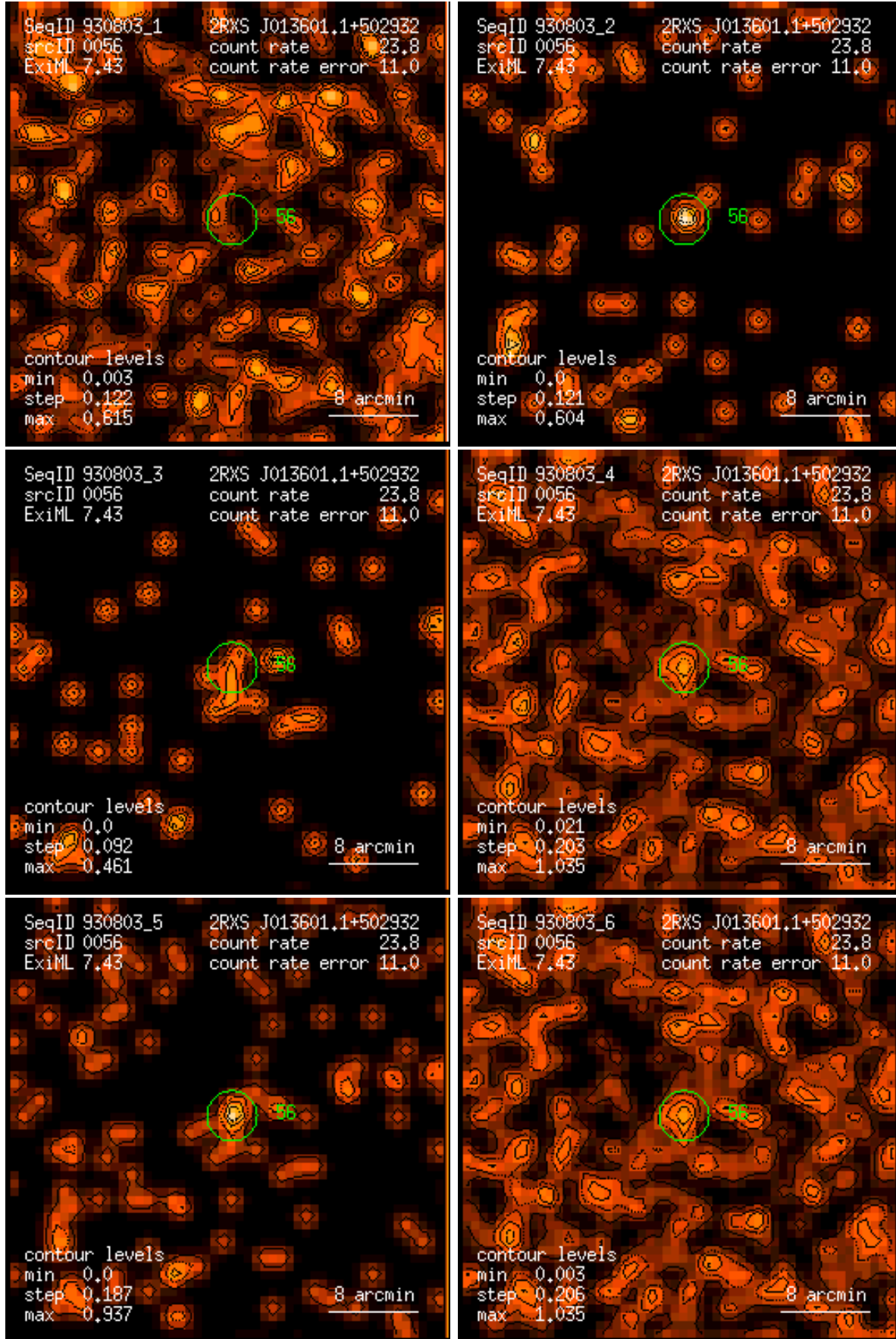
Figure 56: RASS 930803: detection 0056: band rate images, Gaussian filter: (1) PSPC channels 11 – 41, (2) 52 – 90, (3) 91 – 201, (4) 11 – 235, (5) 52 – 201, (6) 11 – 201. Broad band rates in counts/ks. Band rate contour levels in counts/ks/arcmin 2 .
