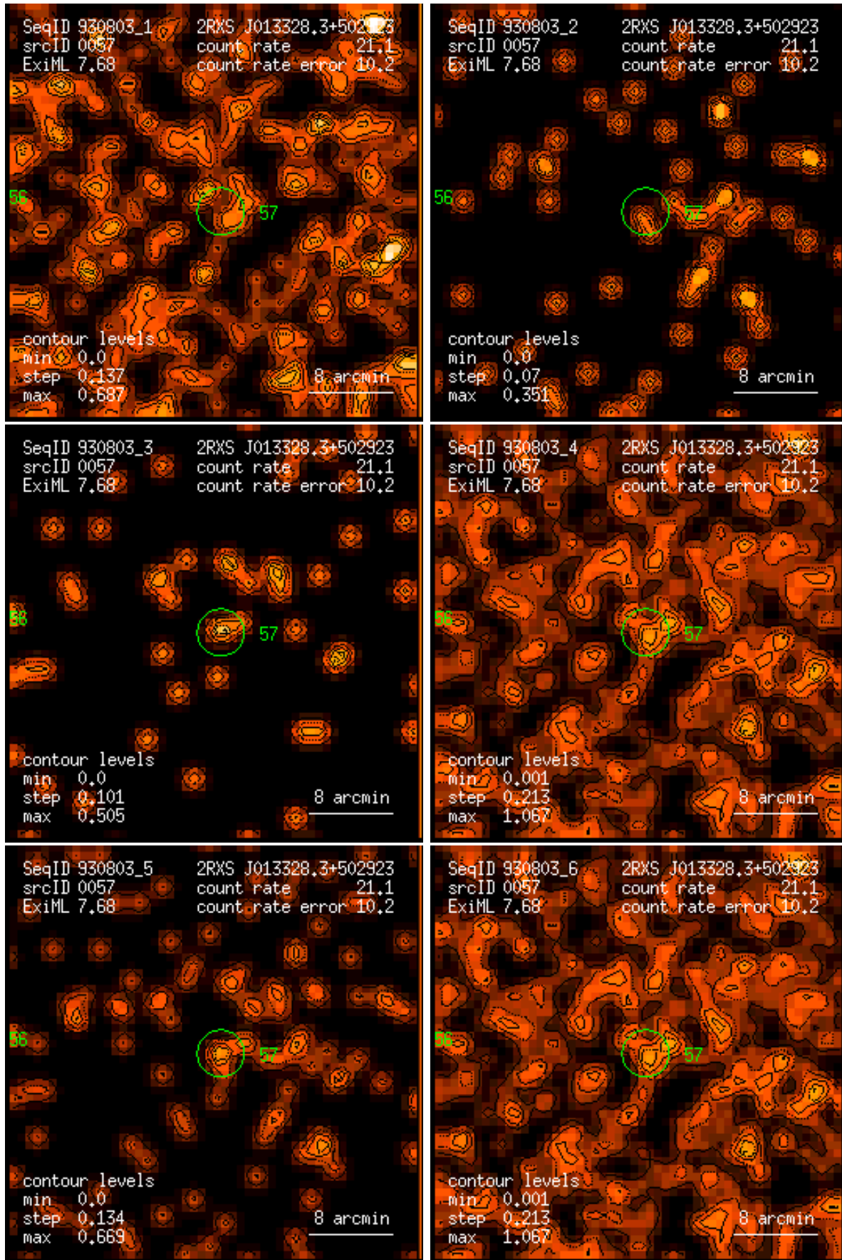
Figure 57: RASS 930803: detection 0057: band rate images, Gaussian filter: (1) PSPC channels 11 – 41, (2) 52 – 90, (3) 91 – 201, (4) 11 – 235, (5) 52 – 201, (6) 11 – 201. Broad band rates in counts/ks. Band rate contour levels in counts/ks/arcmin 2 .
