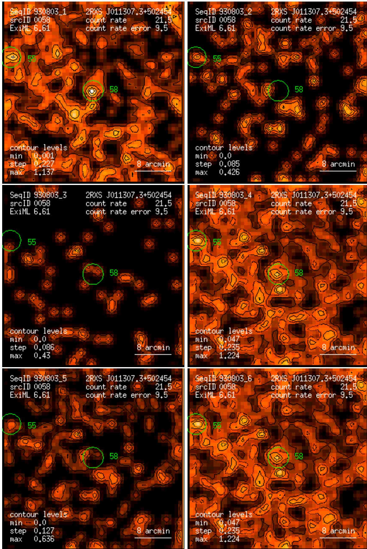
Figure 58: RASS 930803: detection 0058: band rate images, Gaussian filter: (1) PSPC channels 11 – 41, (2) 52 – 90, (3) 91 – 201, (4) 11 – 235, (5) 52 – 201, (6) 11 – 201. Broad band rates in counts/ks. Band rate contour levels in counts/ks/arcmin 2 .
