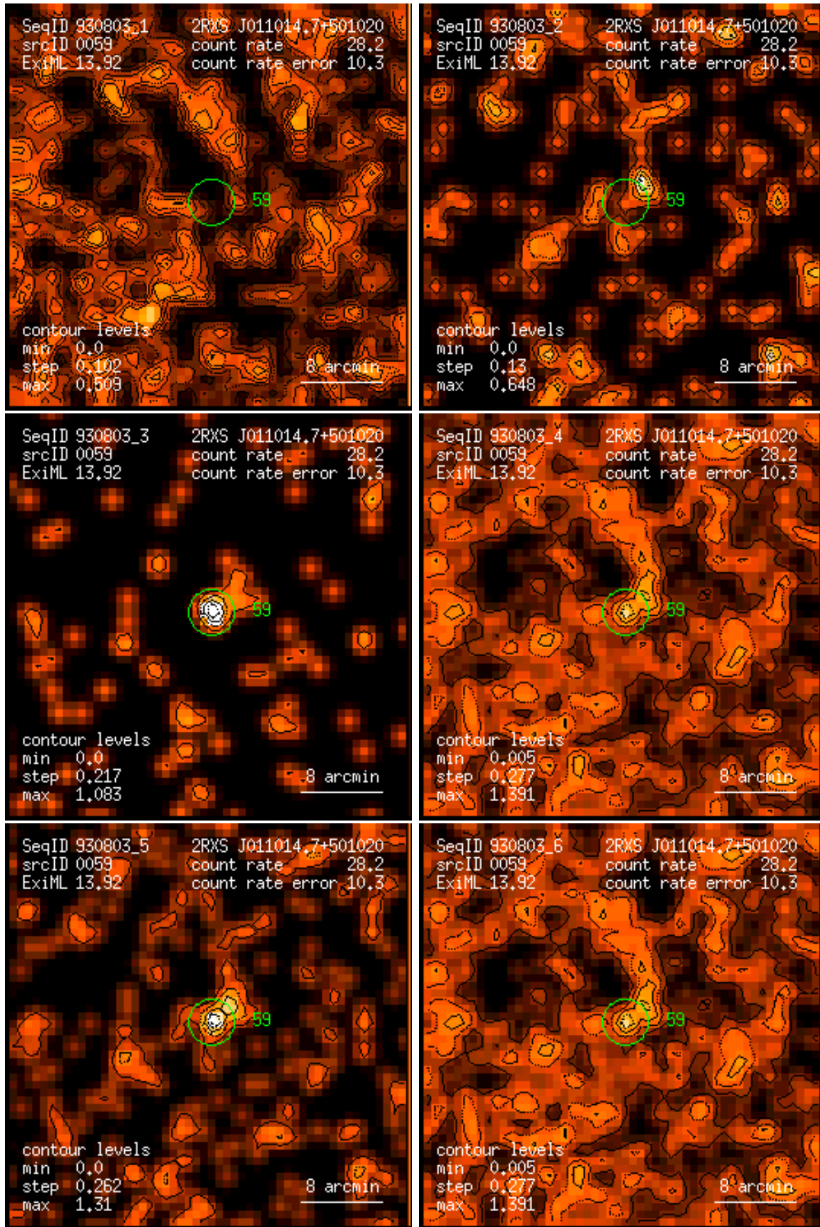
Figure 59: RASS 930803: detection 0059: band rate images, Gaussian filter: (1) PSPC channels 11 – 41, (2) 52 – 90, (3) 91 – 201, (4) 11 – 235, (5) 52 – 201, (6) 11 – 201. Broad band rates in counts/ks. Band rate contour levels in counts/ks/arcmin 2 .
