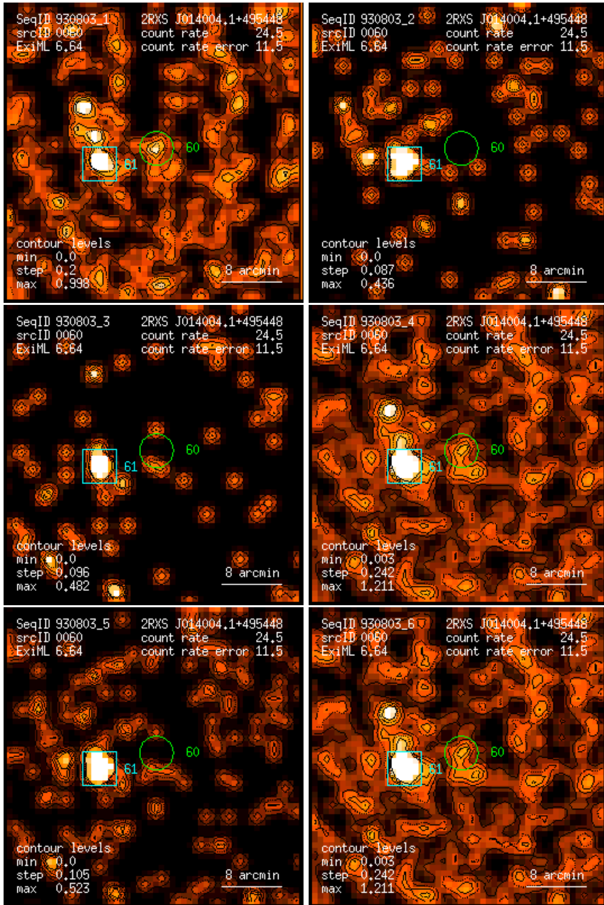
Figure 60: RASS 930803: detection 0060: band rate images, Gaussian filter: (1) PSPC channels 11 – 41, (2) 52 – 90, (3) 91 – 201, (4) 11 – 235, (5) 52 – 201, (6) 11 – 201. Broad band rates in counts/ks. Band rate contour levels in counts/ks/arcmin 2 .
