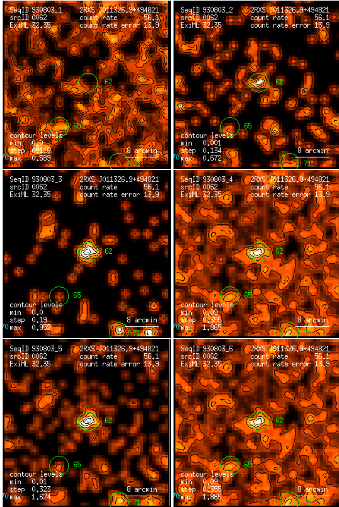
Figure 62: RASS 930803: detection 0062: band rate images, Gaussian filter: (1) PSPC channels 11 – 41, (2) 52 – 90, (3) 91 – 201, (4) 11 – 235, (5) 52 – 201, (6) 11 – 201. Broad band rates in counts/ks. Band rate contour levels in counts/ks/arcmin 2 .
