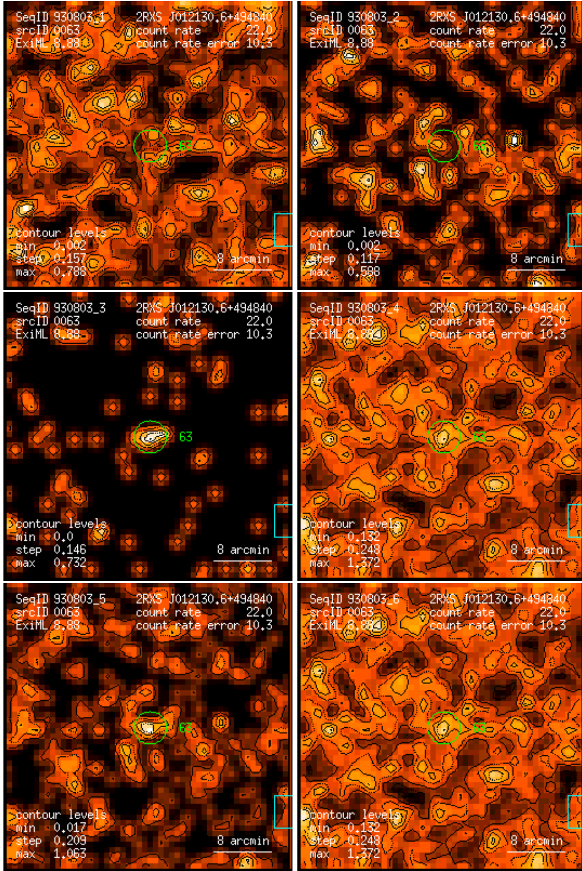
Figure 63: RASS 930803: detection 0063: band rate images, Gaussian filter: (1) PSPC channels 11 – 41, (2) 52 – 90, (3) 91 – 201, (4) 11 – 235, (5) 52 – 201, (6) 11 – 201. Broad band rates in counts/ks. Band rate contour levels in counts/ks/arcmin 2 .
