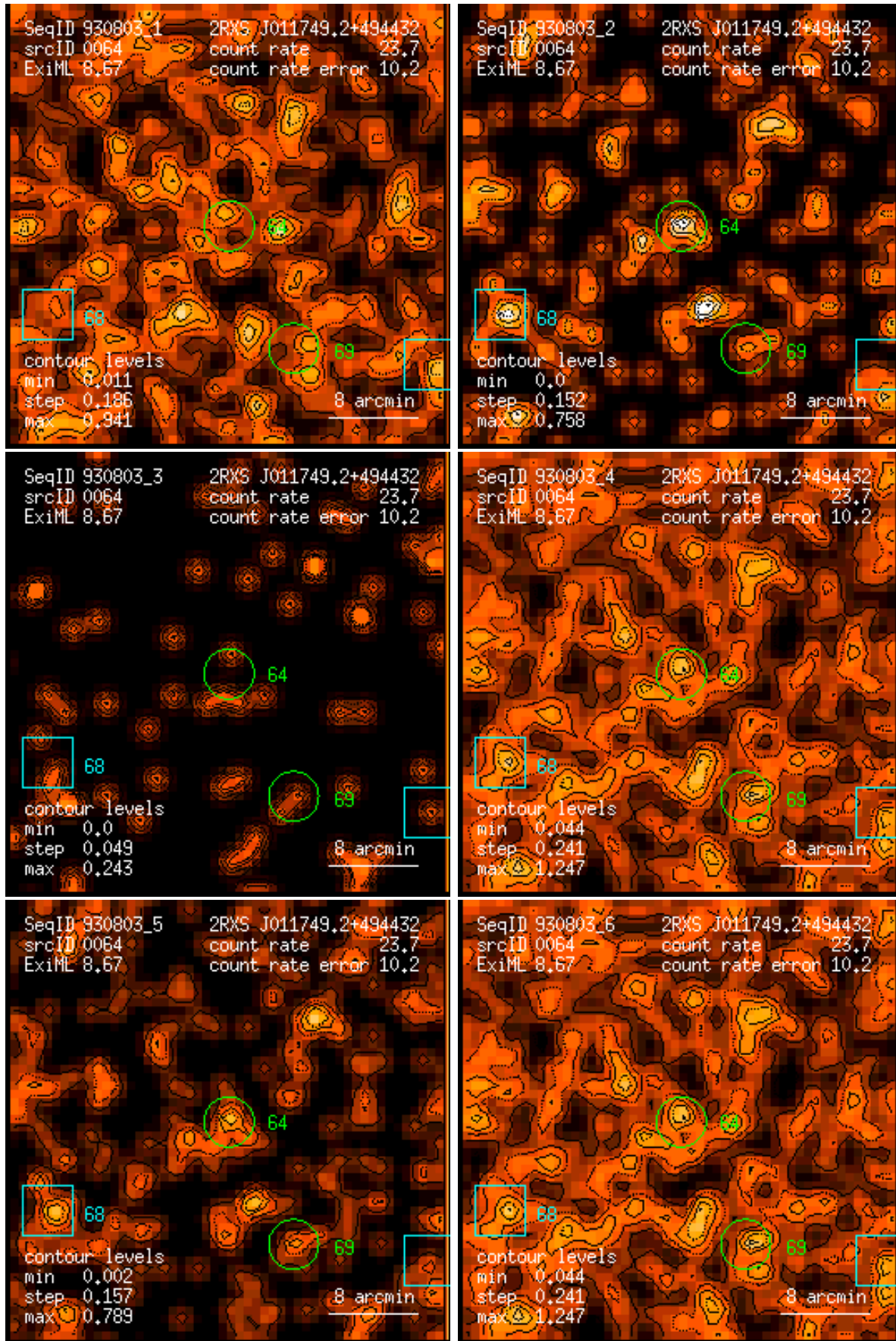
Figure 64: RASS 930803: detection 0064: band rate images, Gaussian filter: (1) PSPC channels 11 – 41, (2) 52 – 90, (3) 91 – 201, (4) 11 – 235, (5) 52 – 201, (6) 11 – 201. Broad band rates in counts/ks. Band rate contour levels in counts/ks/arcmin 2 .
