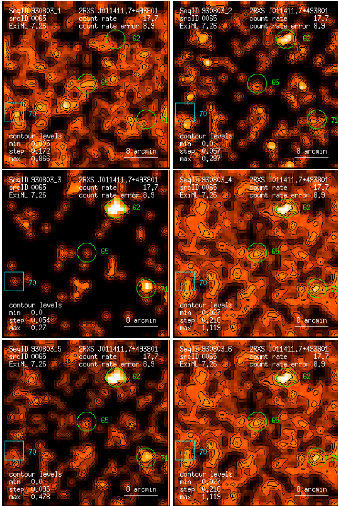
Figure 65: RASS 930803: detection 0065: band rate images, Gaussian filter: (1) PSPC channels 11 – 41, (2) 52 – 90, (3) 91 – 201, (4) 11 – 235, (5) 52 – 201, (6) 11 – 201. Broad band rates in counts/ks. Band rate contour levels in counts/ks/arcmin 2 .
