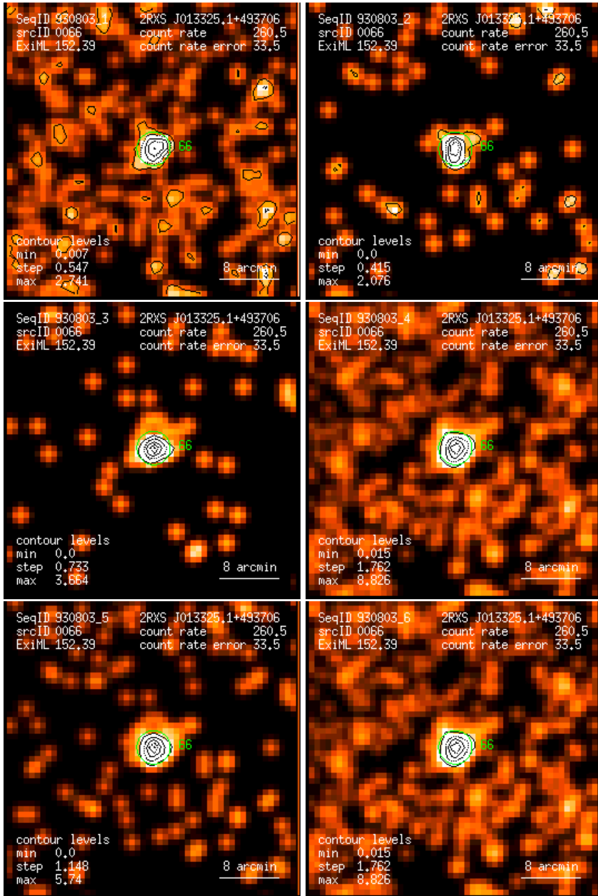
Figure 66: RASS 930803: detection 0066: band rate images, Gaussian filter: (1) PSPC channels 11 – 41, (2) 52 – 90, (3) 91 – 201, (4) 11 – 235, (5) 52 – 201, (6) 11 – 201. Broad band rates in counts/ks. Band rate contour levels in counts/ks/arcmin 2 .
