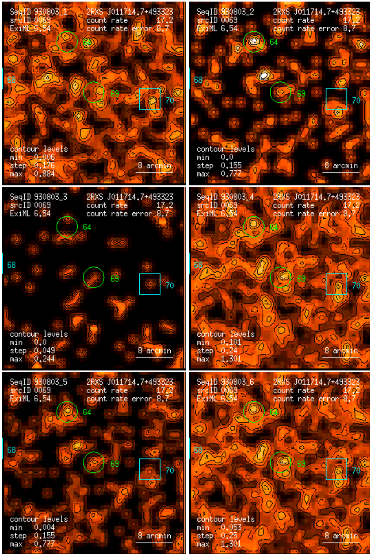
Figure 69: RASS 930803: detection 0069: band rate images, Gaussian filter: (1) PSPC channels 11 – 41, (2) 52 – 90, (3) 91 – 201, (4) 11 – 235, (5) 52 – 201, (6) 11 – 201. Broad band rates in counts/ks. Band rate contour levels in counts/ks/arcmin 2 .
