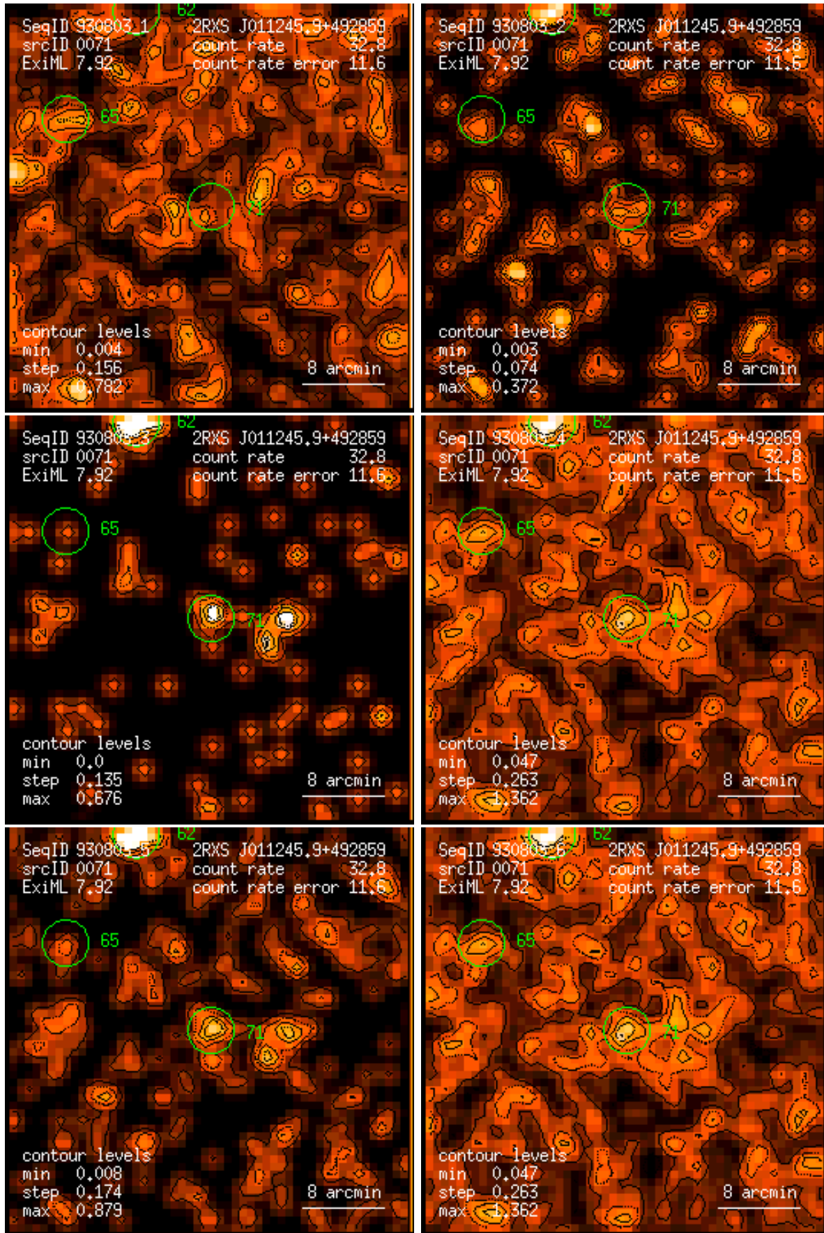
Figure 71: RASS 930803: detection 0071: band rate images, Gaussian filter: (1) PSPC channels 11 – 41, (2) 52 – 90, (3) 91 – 201, (4) 11 – 235, (5) 52 – 201, (6) 11 – 201. Broad band rates in counts/ks. Band rate contour levels in counts/ks/arcmin 2 .
