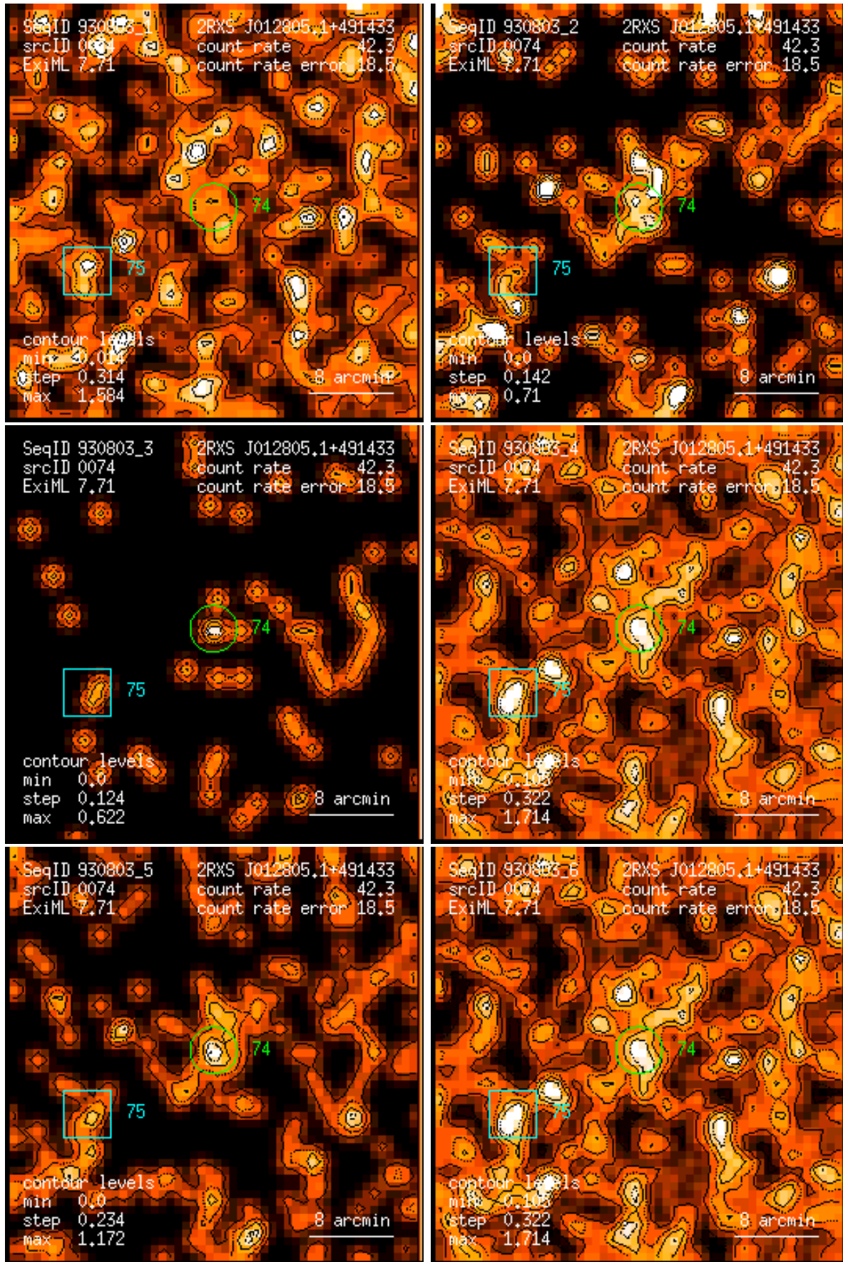
Figure 74: RASS 930803: detection 0074: band rate images, Gaussian filter: (1) PSPC channels 11 – 41, (2) 52 – 90, (3) 91 – 201, (4) 11 – 235, (5) 52 – 201, (6) 11 – 201. Broad band rates in counts/ks. Band rate contour levels in counts/ks/arcmin 2 .
