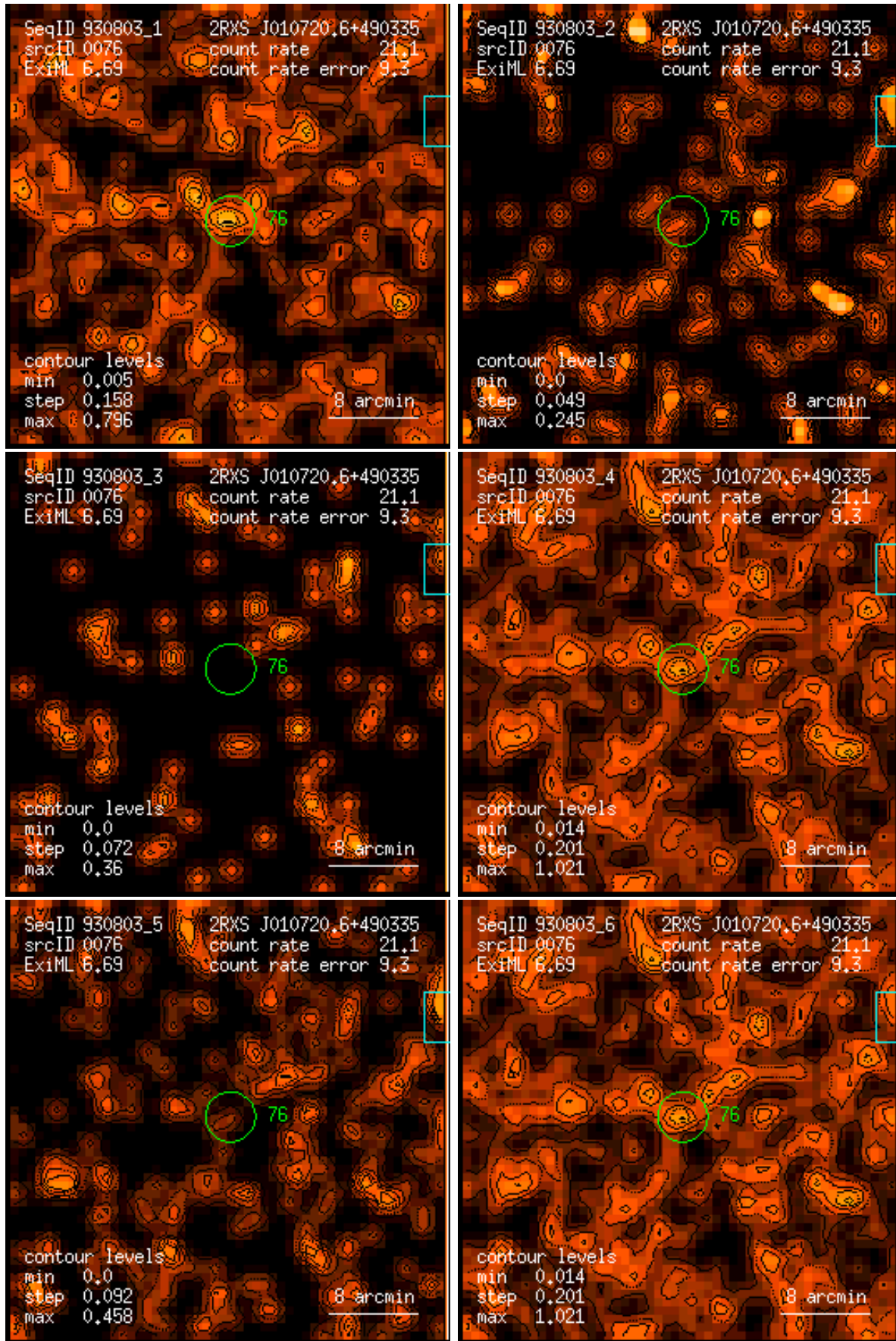
Figure 76: RASS 930803: detection 0076: band rate images, Gaussian filter: (1) PSPC channels 11 – 41, (2) 52 – 90, (3) 91 – 201, (4) 11 – 235, (5) 52 – 201, (6) 11 – 201. Broad band rates in counts/ks. Band rate contour levels in counts/ks/arcmin 2 .
