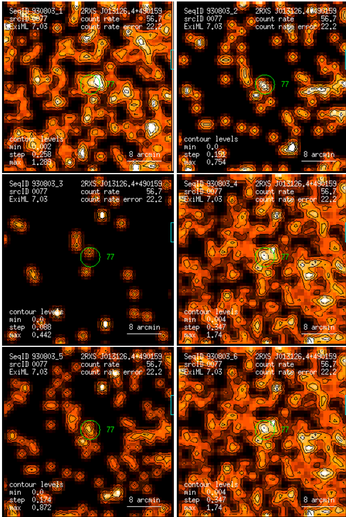
Figure 77: RASS 930803: detection 0077: band rate images, Gaussian filter: (1) PSPC channels 11 – 41, (2) 52 – 90, (3) 91 – 201, (4) 11 – 235, (5) 52 – 201, (6) 11 – 201. Broad band rates in counts/ks. Band rate contour levels in counts/ks/arcmin 2 .
