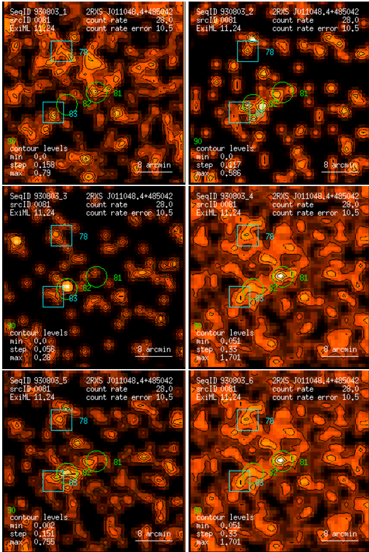
Figure 81: RASS 930803: detection 0081: band rate images, Gaussian filter: (1) PSPC channels 11 – 41, (2) 52 – 90, (3) 91 – 201, (4) 11 – 235, (5) 52 – 201, (6) 11 – 201. Broad band rates in counts/ks. Band rate contour levels in counts/ks/arcmin 2 .
