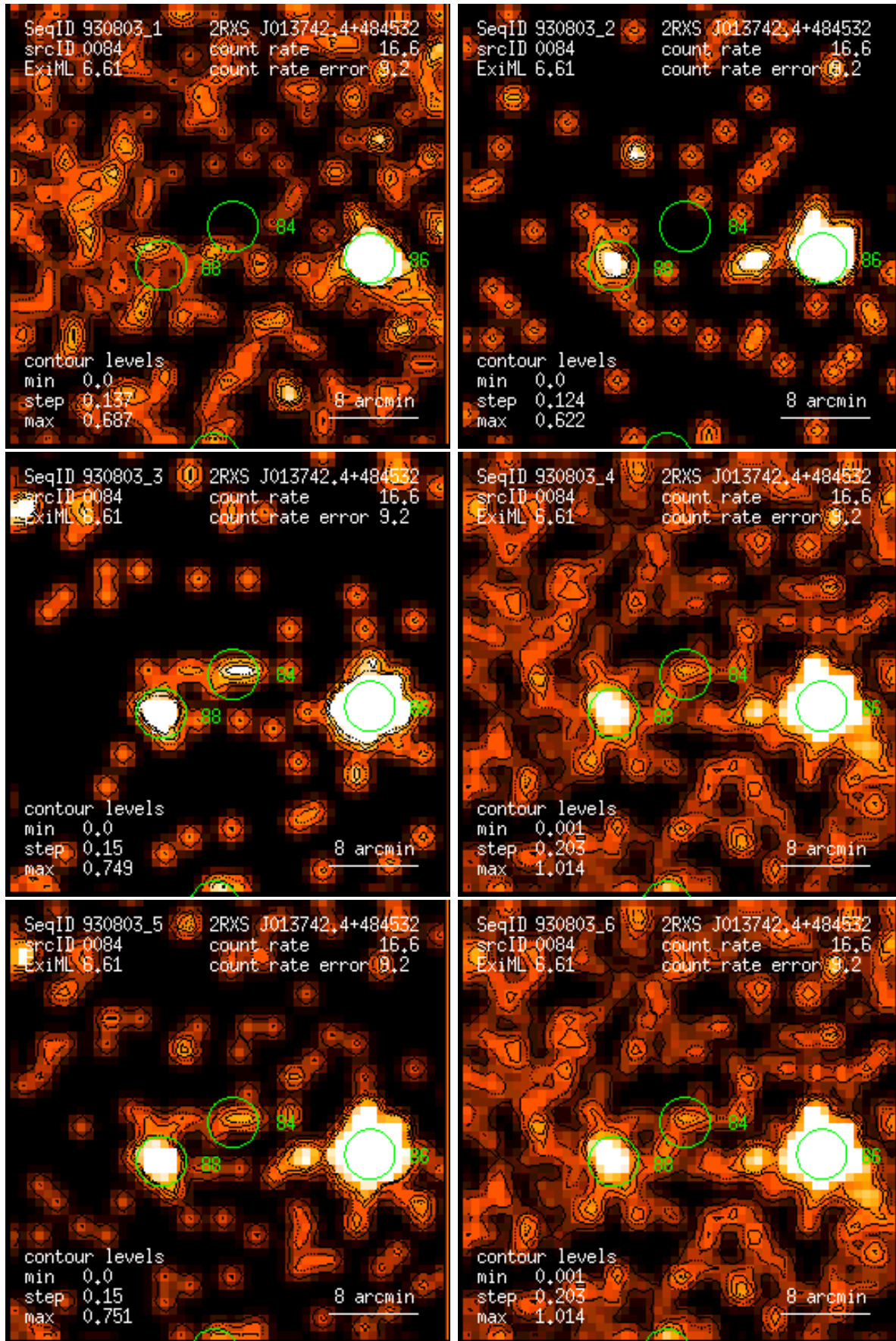
Figure 84: RASS 930803: detection 0084: band rate images, Gaussian filter: (1) PSPC channels 11 – 41, (2) 52 – 90, (3) 91 – 201, (4) 11 – 235, (5) 52 – 201, (6) 11 – 201. Broad band rates in counts/ks. Band rate contour levels in counts/ks/arcmin 2 .
