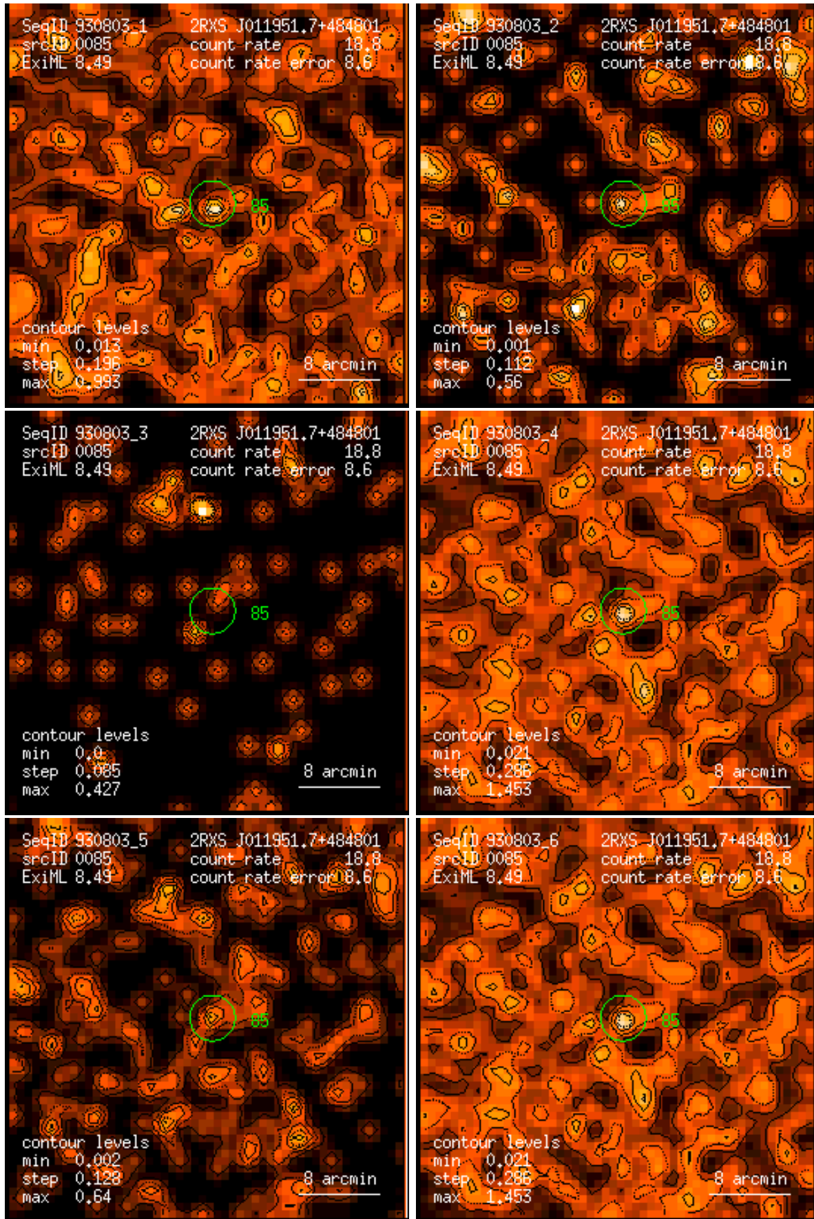
Figure 85: RASS 930803: detection 0085: band rate images, Gaussian filter: (1) PSPC channels 11 – 41, (2) 52 – 90, (3) 91 – 201, (4) 11 – 235, (5) 52 – 201, (6) 11 – 201. Broad band rates in counts/ks. Band rate contour levels in counts/ks/arcmin 2 .
