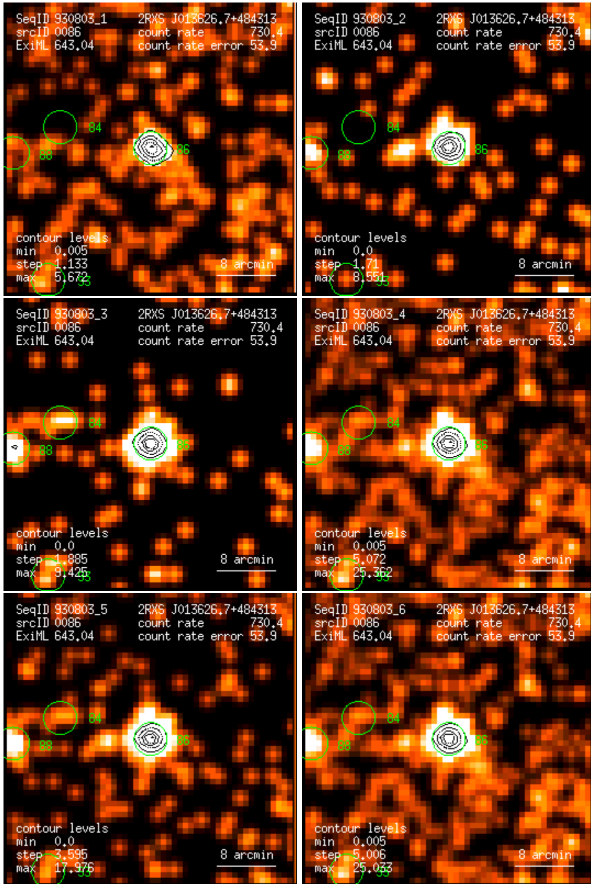
Figure 86: RASS 930803: detection 0086: band rate images, Gaussian filter: (1) PSPC channels 11 – 41, (2) 52 – 90, (3) 91 – 201, (4) 11 – 235, (5) 52 – 201, (6) 11 – 201. Broad band rates in counts/ks. Band rate contour levels in counts/ks/arcmin 2 .
