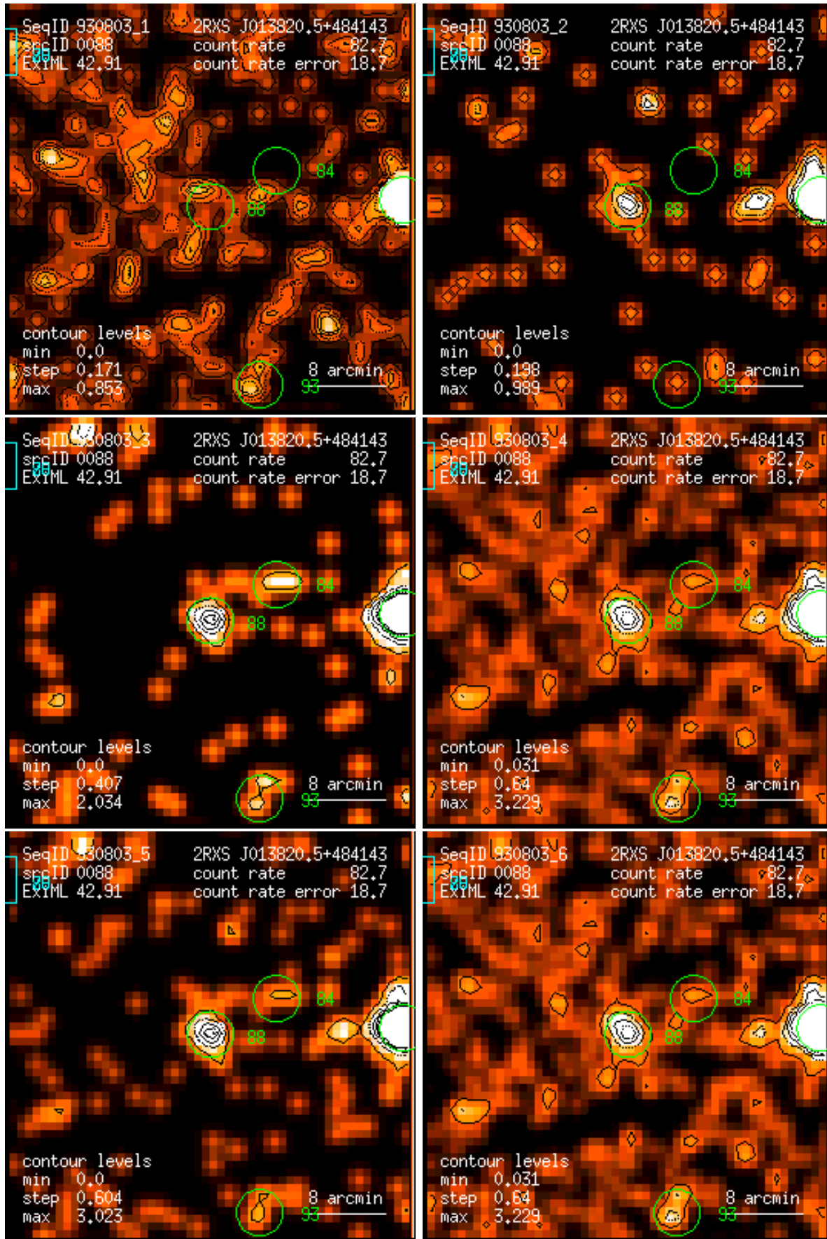
Figure 88: RASS 930803: detection 0088: band rate images, Gaussian filter: (1) PSPC channels 11 – 41, (2) 52 – 90, (3) 91 – 201, (4) 11 – 235, (5) 52 – 201, (6) 11 – 201. Broad band rates in counts/ks. Band rate contour levels in counts/ks/arcmin 2 .
