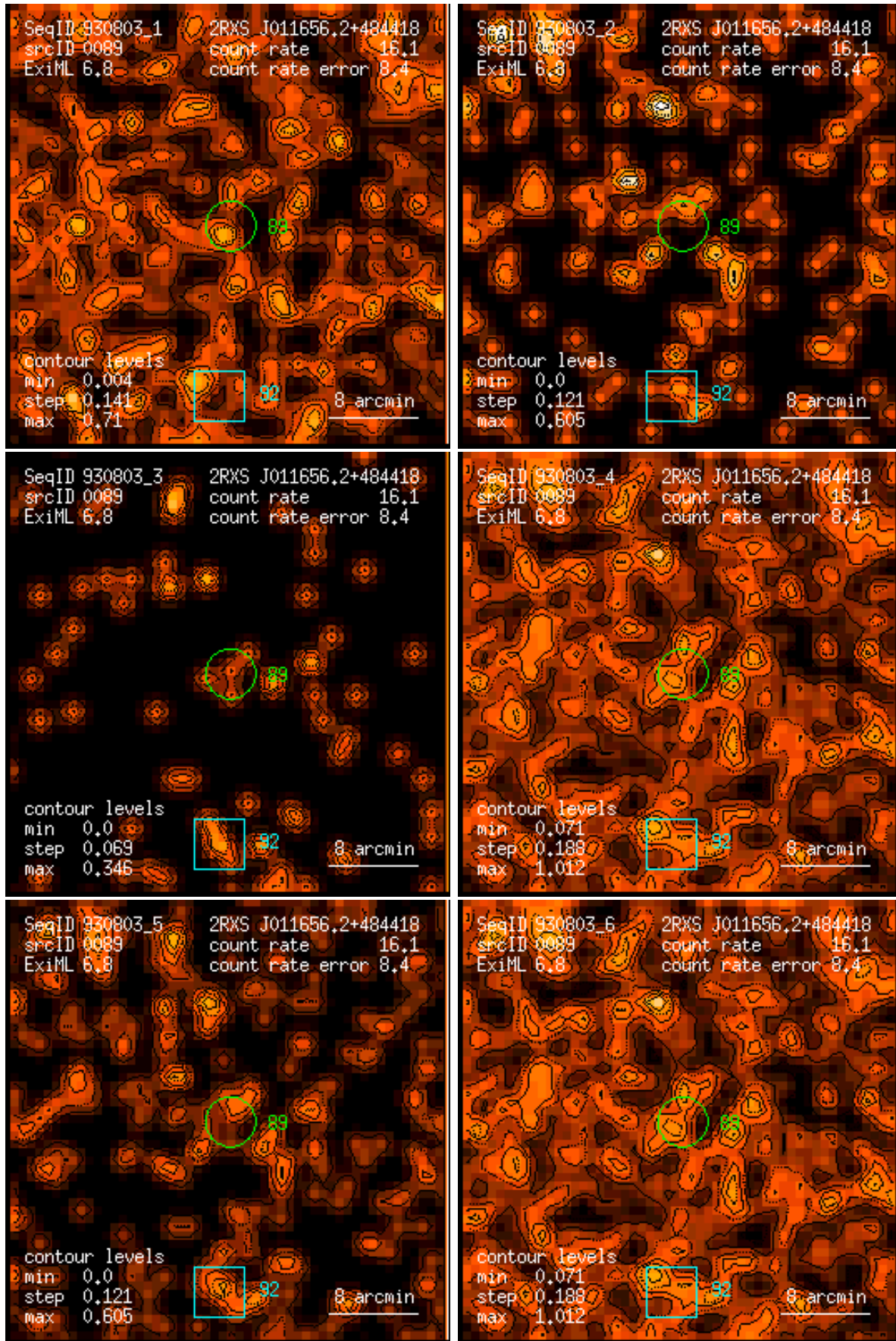
Figure 89: RASS 930803: detection 0089: band rate images, Gaussian filter: (1) PSPC channels 11 – 41, (2) 52 – 90, (3) 91 – 201, (4) 11 – 235, (5) 52 – 201, (6) 11 – 201. Broad band rates in counts/ks. Band rate contour levels in counts/ks/arcmin 2 .
