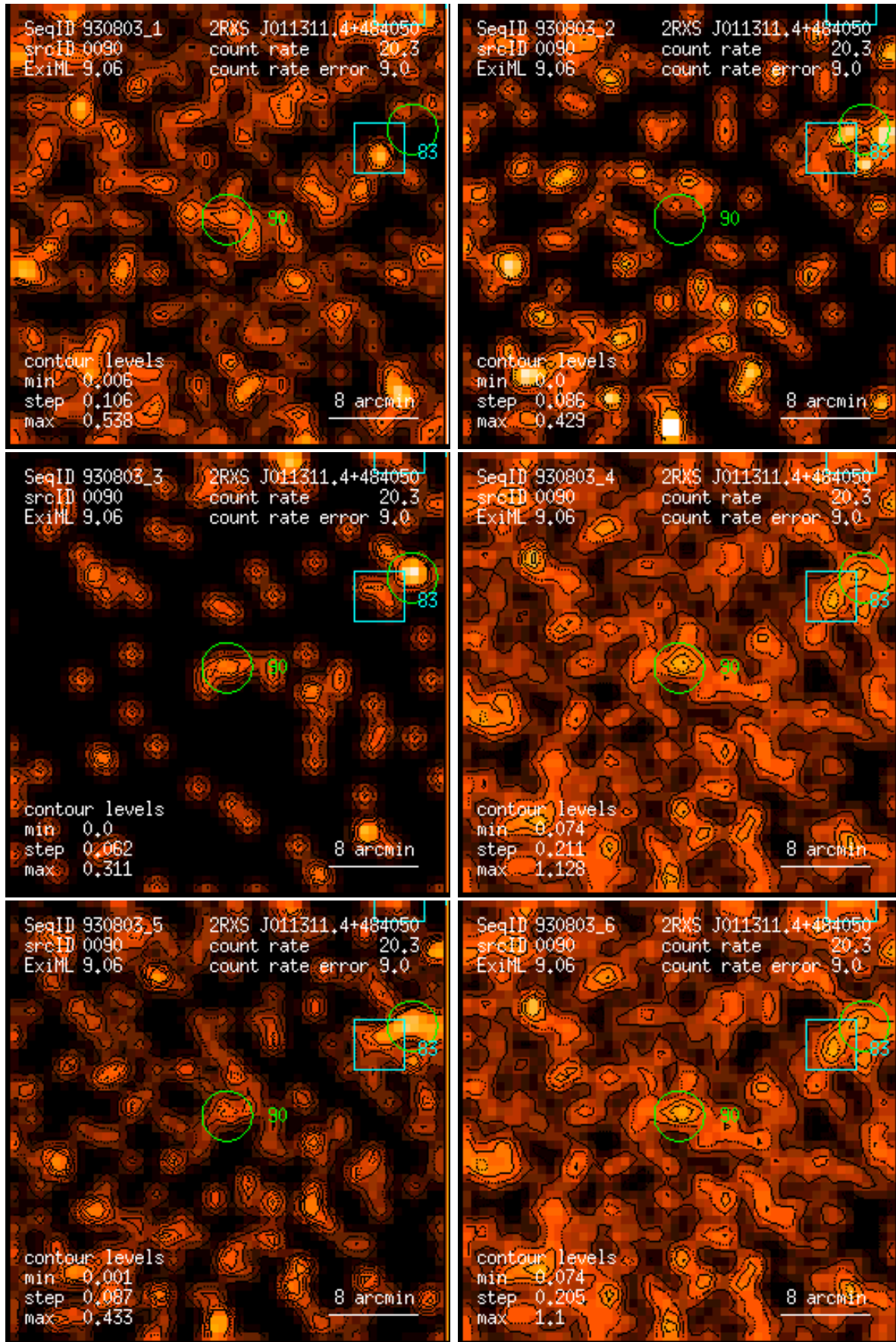
Figure 90: RASS 930803: detection 0090: band rate images, Gaussian filter: (1) PSPC channels 11 – 41, (2) 52 – 90, (3) 91 – 201, (4) 11 – 235, (5) 52 – 201, (6) 11 – 201. Broad band rates in counts/ks. Band rate contour levels in counts/ks/arcmin 2 .
