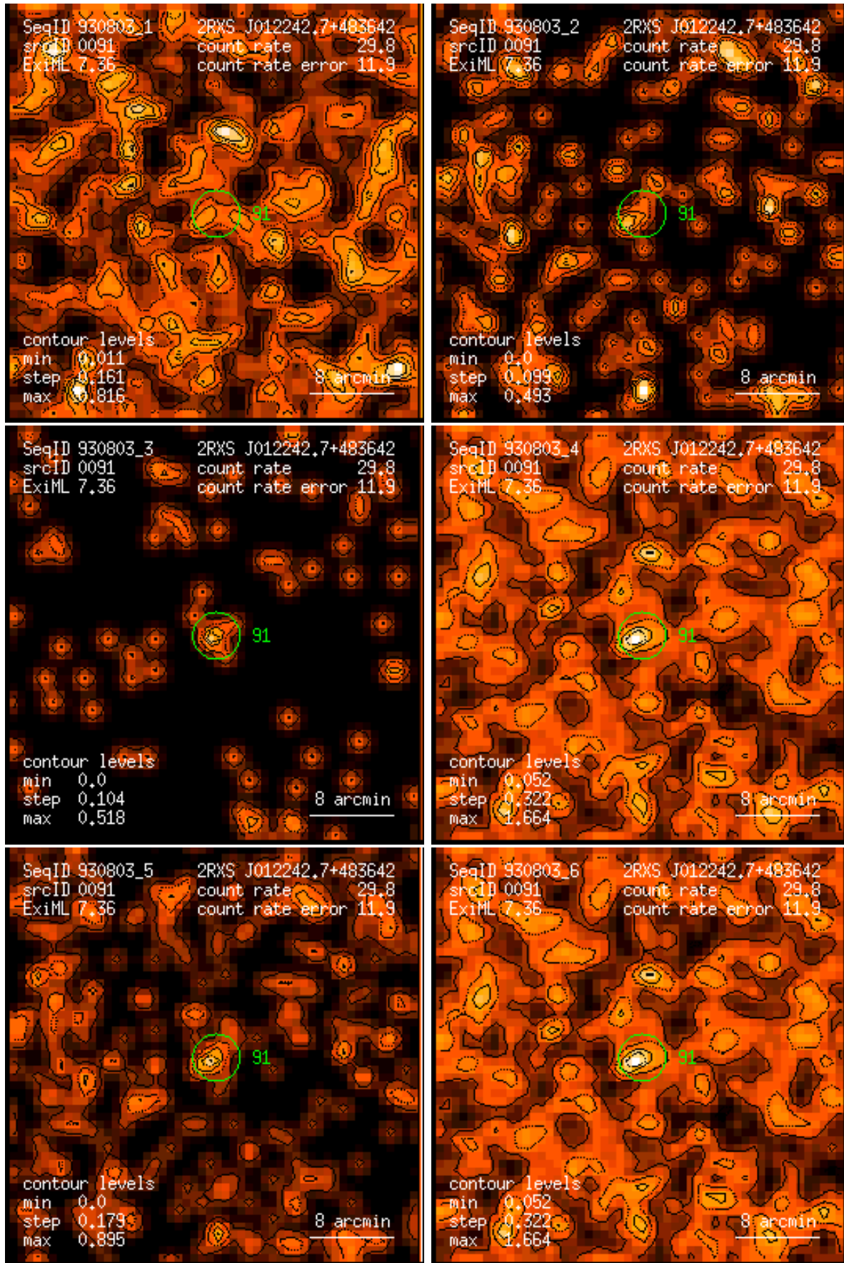
Figure 91: RASS 930803: detection 0091: band rate images, Gaussian filter: (1) PSPC channels 11 – 41, (2) 52 – 90, (3) 91 – 201, (4) 11 – 235, (5) 52 – 201, (6) 11 – 201. Broad band rates in counts/ks. Band rate contour levels in counts/ks/arcmin 2 .
