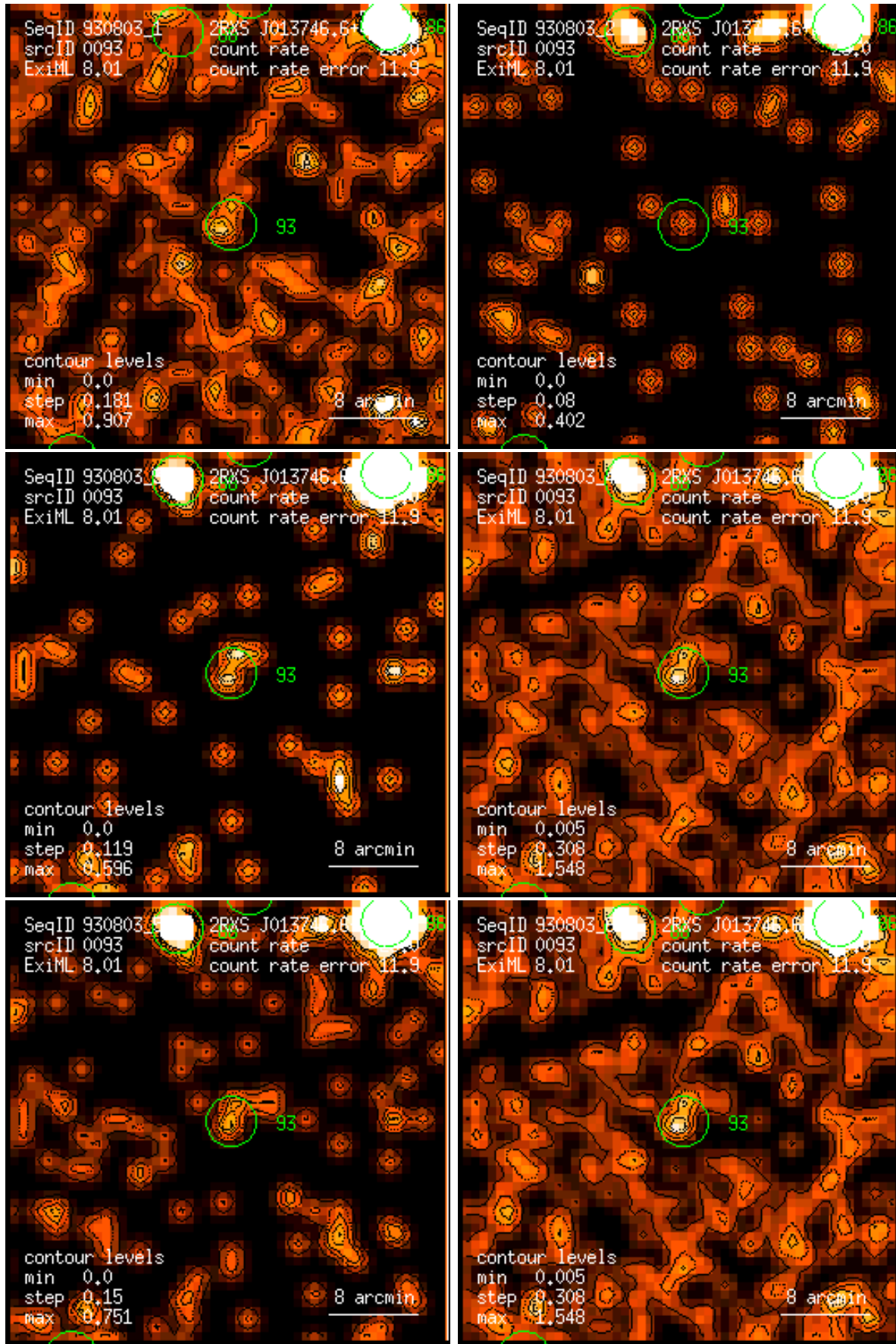
Figure 93: RASS 930803: detection 0093: band rate images, Gaussian filter: (1) PSPC channels 11 – 41, (2) 52 – 90, (3) 91 – 201, (4) 11 – 235, (5) 52 – 201, (6) 11 – 201. Broad band rates in counts/ks. Band rate contour levels in counts/ks/arcmin 2 .
