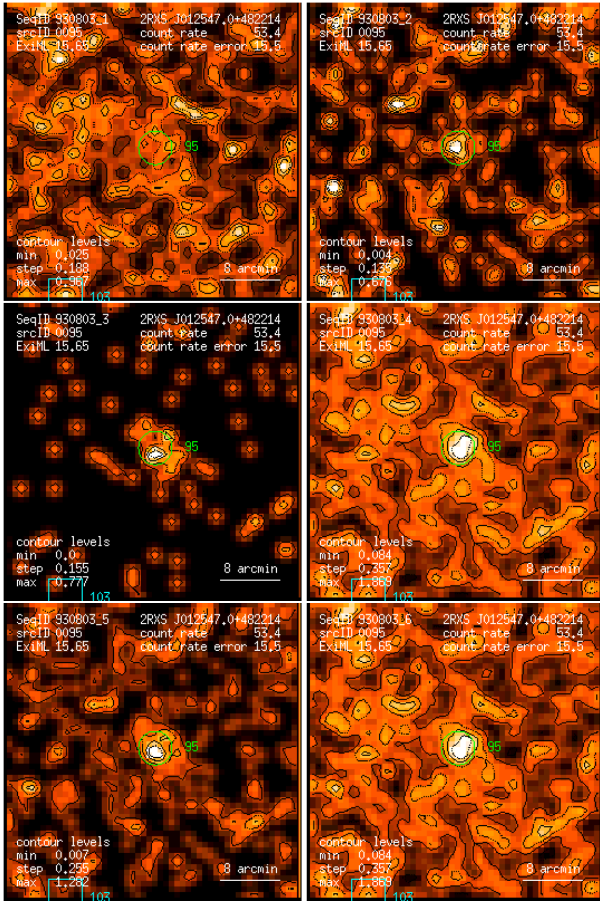
Figure 95: RASS 930803: detection 0095: band rate images, Gaussian filter: (1) PSPC channels 11 – 41, (2) 52 – 90, (3) 91 – 201, (4) 11 – 235, (5) 52 – 201, (6) 11 – 201. Broad band rates in counts/ks. Band rate contour levels in counts/ks/arcmin 2 .
