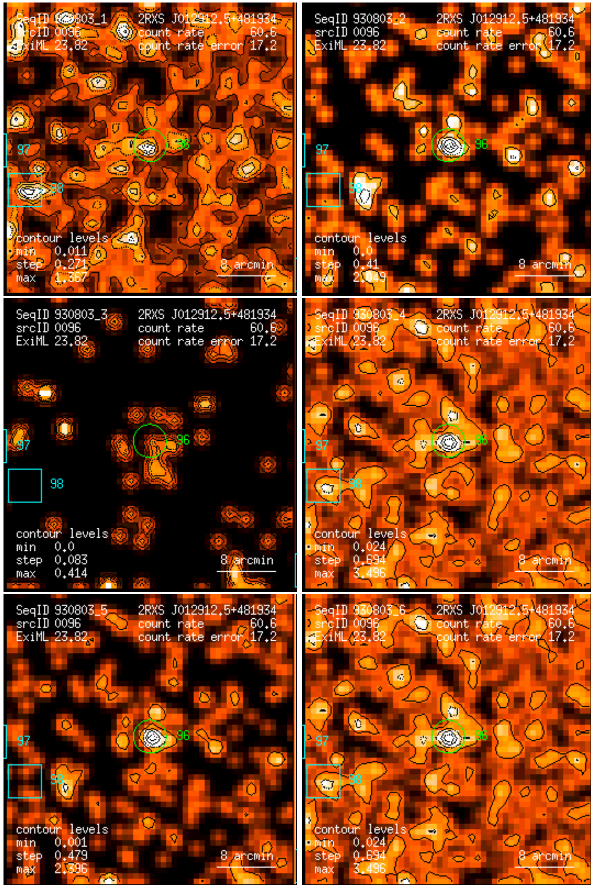
Figure 96: RASS 930803: detection 0096: band rate images, Gaussian filter: (1) PSPC channels 11 – 41, (2) 52 – 90, (3) 91 – 201, (4) 11 – 235, (5) 52 – 201, (6) 11 – 201. Broad band rates in counts/ks. Band rate contour levels in counts/ks/arcmin 2 .
