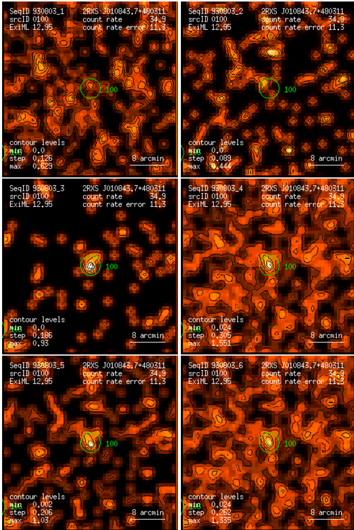
Figure 100: RASS 930803: detection 0100: band rate images, Gaussian filter: (1) PSPC channels 11 – 41, (2) 52 – 90, (3) 91 – 201, (4) 11 – 235, (5) 52 – 201, (6) 11 – 201. Broad band rates in counts/ks. Band rate contour levels in counts/ks/arcmin 2 .
