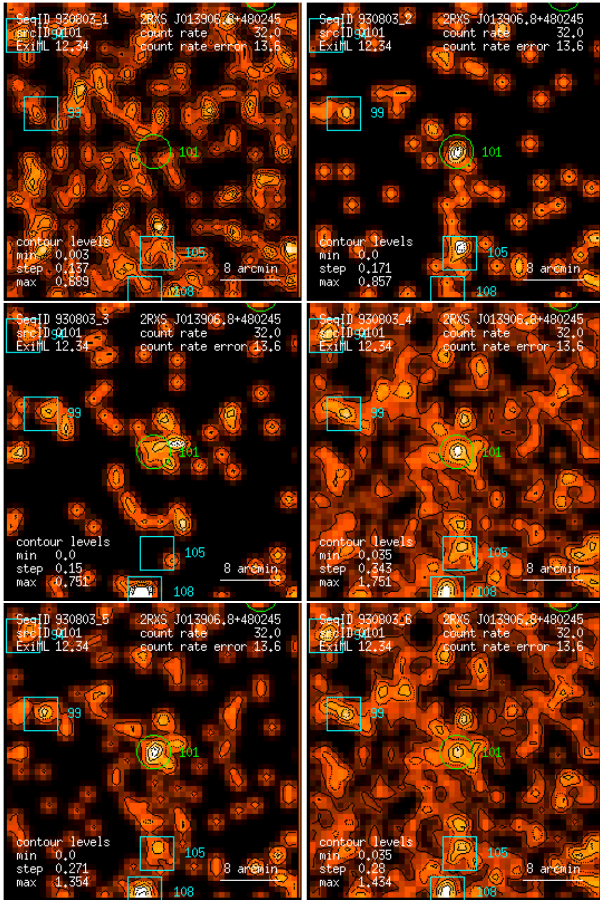
Figure 101: RASS 930803: detection 0101: band rate images, Gaussian filter: (1) PSPC channels 11 – 41, (2) 52 – 90, (3) 91 – 201, (4) 11 – 235, (5) 52 – 201, (6) 11 – 201. Broad band rates in counts/ks. Band rate contour levels in counts/ks/arcmin 2 .
