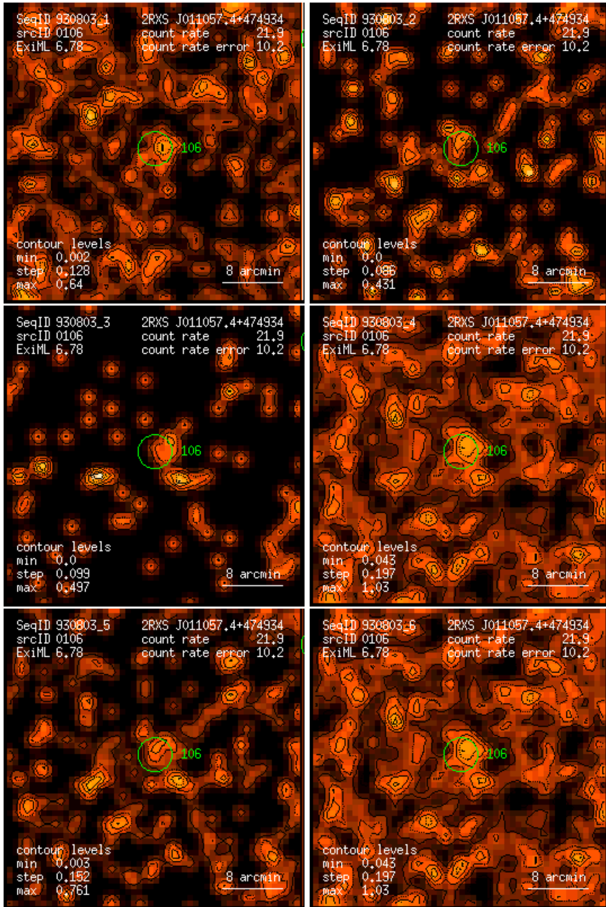
Figure 106: RASS 930803: detection 0106: band rate images, Gaussian filter: (1) PSPC channels 11 – 41, (2) 52 – 90, (3) 91 – 201, (4) 11 – 235, (5) 52 – 201, (6) 11 – 201. Broad band rates in counts/ks. Band rate contour levels in counts/ks/arcmin 2 .
