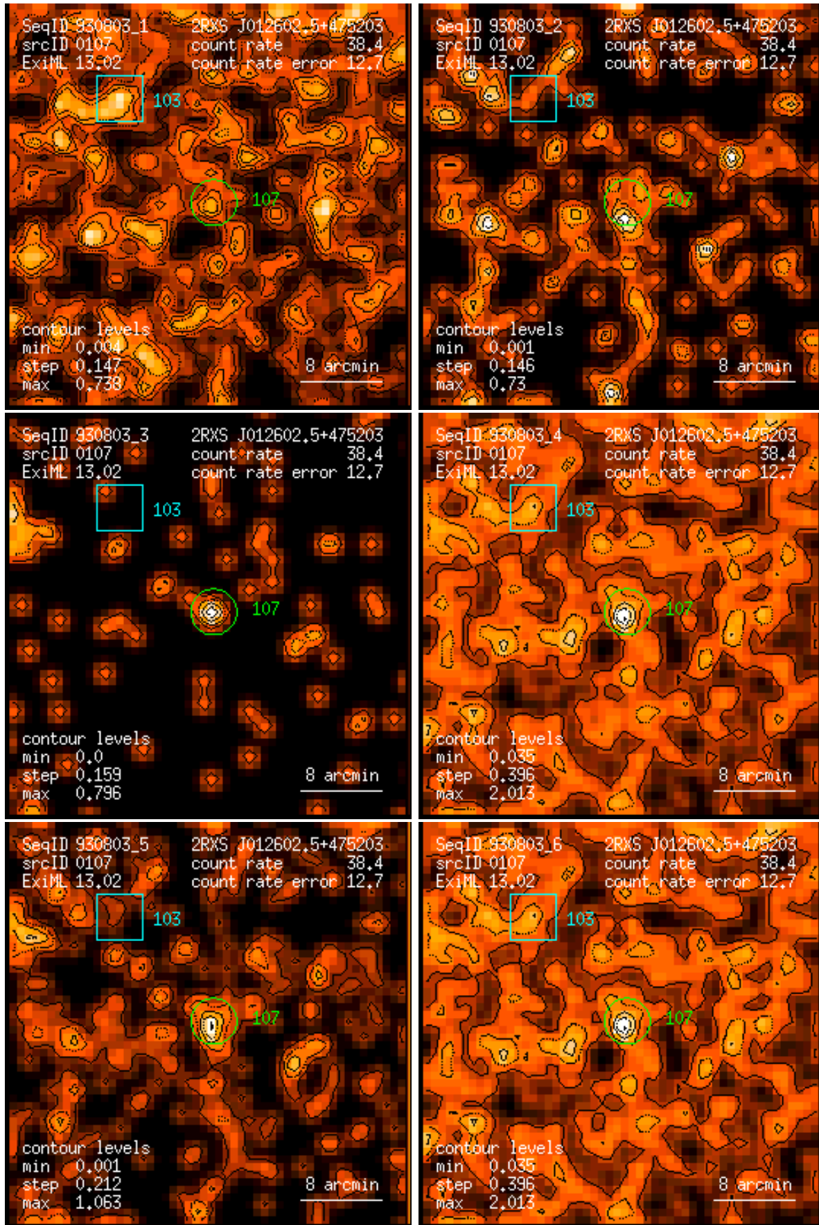
Figure 107: RASS 930803: detection 0107: band rate images, Gaussian filter: (1) PSPC channels 11 – 41, (2) 52 – 90, (3) 91 – 201, (4) 11 – 235, (5) 52 – 201, (6) 11 – 201. Broad band rates in counts/ks. Band rate contour levels in counts/ks/arcmin 2 .
