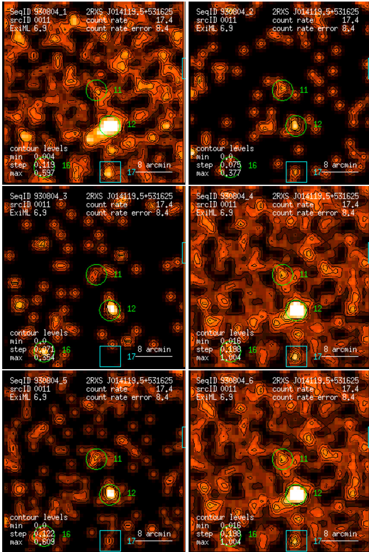
Figure 11: RASS 930804: detection 0011: band rate images, Gaussian filter: (1) PSPC channels 11 – 41, (2) 52 – 90, (3) 91 – 201, (4) 11 – 235, (5) 52 – 201, (6) 11 – 201. Broad band rates in counts/ks. Band rate contour levels in counts/ks/arcmin 2 .
