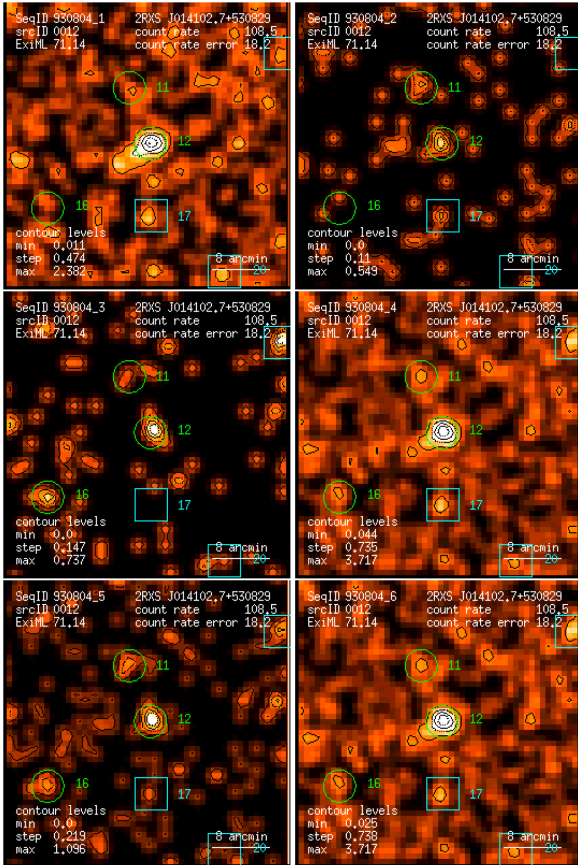
Figure 12: RASS 930804: detection 0012: band rate images, Gaussian filter: (1) PSPC channels 11 – 41, (2) 52 – 90, (3) 91 – 201, (4) 11 – 235, (5) 52 – 201, (6) 11 – 201. Broad band rates in counts/ks. Band rate contour levels in counts/ks/arcmin 2 .
