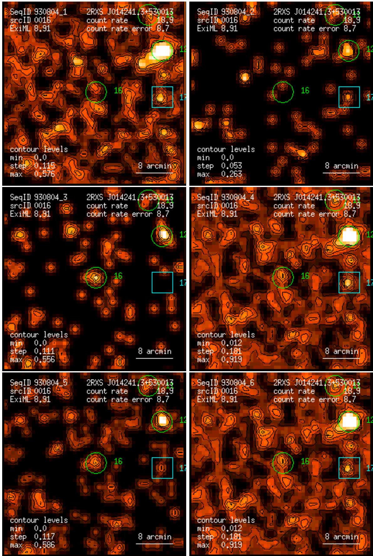
Figure 16: RASS 930804: detection 0016: band rate images, Gaussian filter: (1) PSPC channels 11 – 41, (2) 52 – 90, (3) 91 – 201, (4) 11 – 235, (5) 52 – 201, (6) 11 – 201. Broad band rates in counts/ks. Band rate contour levels in counts/ks/arcmin 2 .
