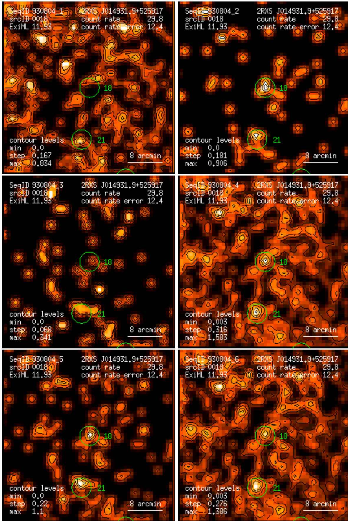
Figure 18: RASS 930804: detection 0018: band rate images, Gaussian filter: (1) PSPC channels 11 – 41, (2) 52 – 90, (3) 91 – 201, (4) 11 – 235, (5) 52 – 201, (6) 11 – 201. Broad band rates in counts/ks. Band rate contour levels in counts/ks/arcmin 2 .
