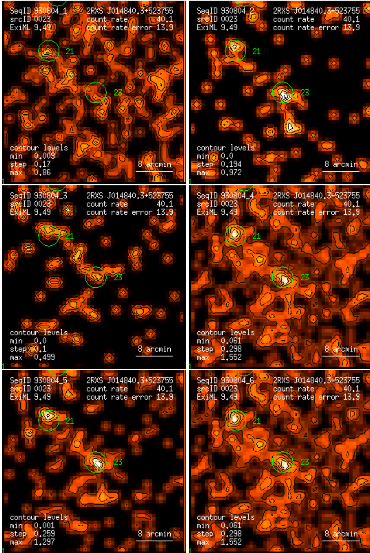
Figure 23: RASS 930804: detection 0023: band rate images, Gaussian filter: (1) PSPC channels 11 – 41, (2) 52 – 90, (3) 91 – 201, (4) 11 – 235, (5) 52 – 201, (6) 11 – 201. Broad band rates in counts/ks. Band rate contour levels in counts/ks/arcmin 2 .
