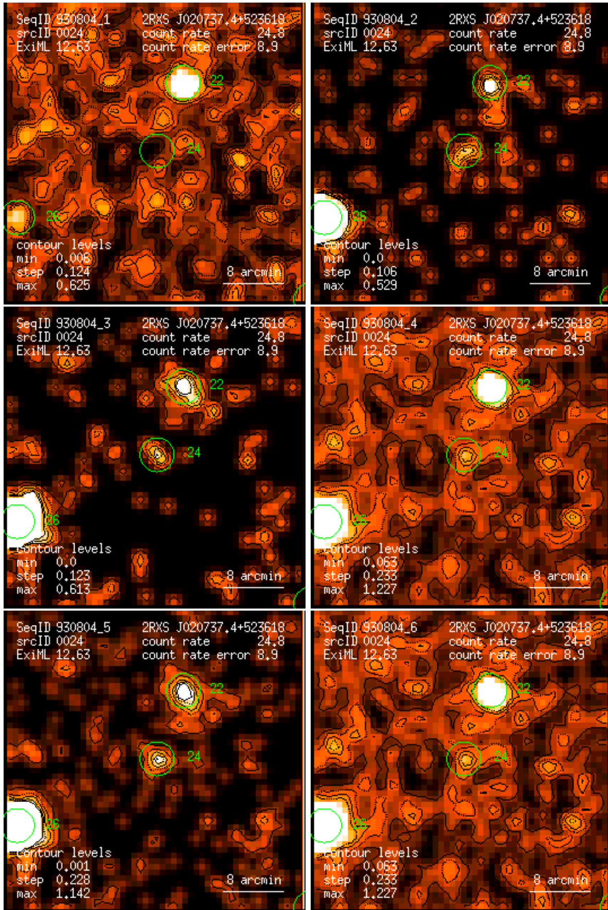
Figure 24: RASS 930804: detection 0024: band rate images, Gaussian filter: (1) PSPC channels 11 – 41, (2) 52 – 90, (3) 91 – 201, (4) 11 – 235, (5) 52 – 201, (6) 11 – 201. Broad band rates in counts/ks. Band rate contour levels in counts/ks/arcmin 2 .
