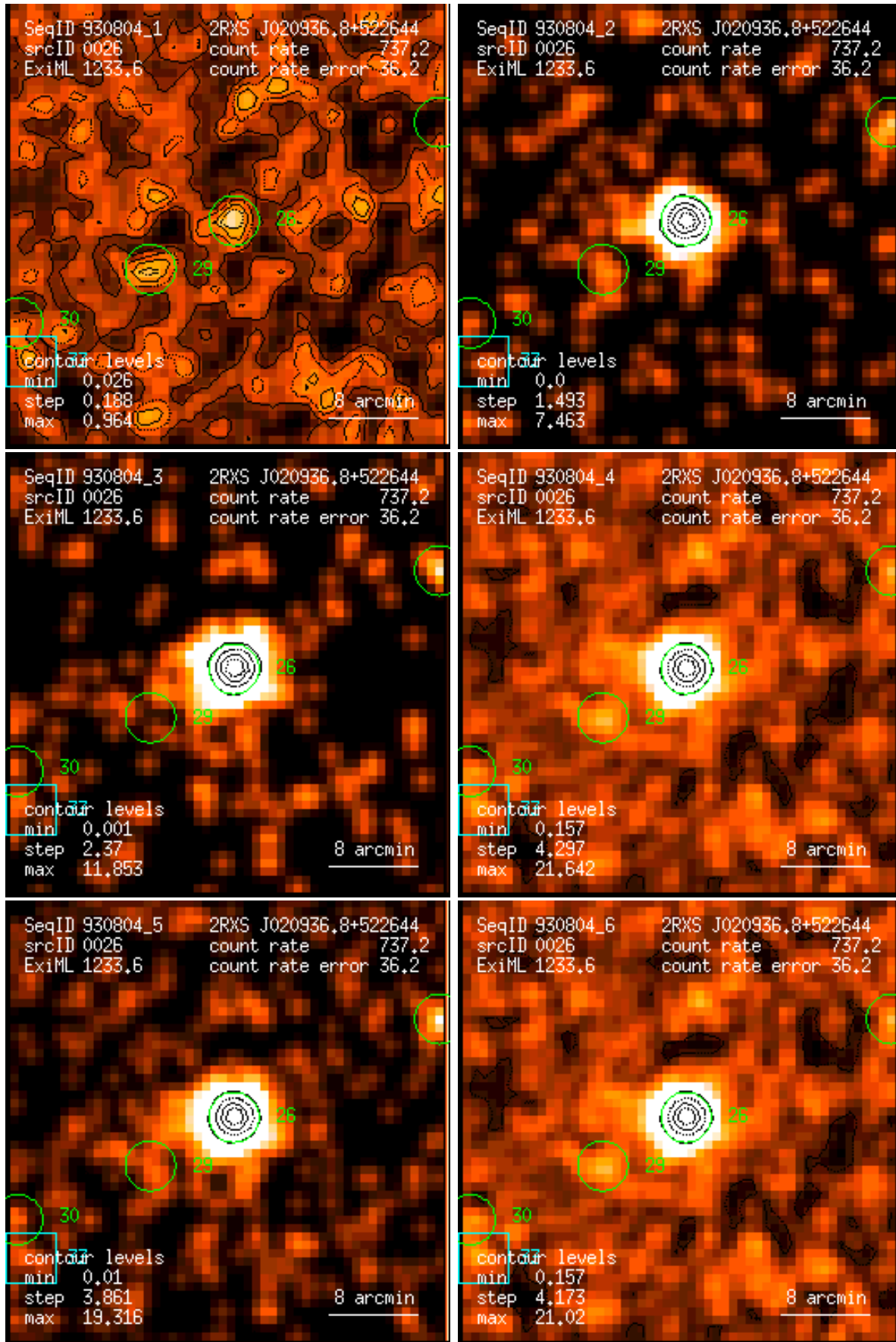
Figure 26: RASS 930804: detection 0026: band rate images, Gaussian filter: (1) PSPC channels 11 – 41, (2) 52 – 90, (3) 91 – 201, (4) 11 – 235, (5) 52 – 201, (6) 11 – 201. Broad band rates in counts/ks. Band rate contour levels in counts/ks/arcmin 2 .
