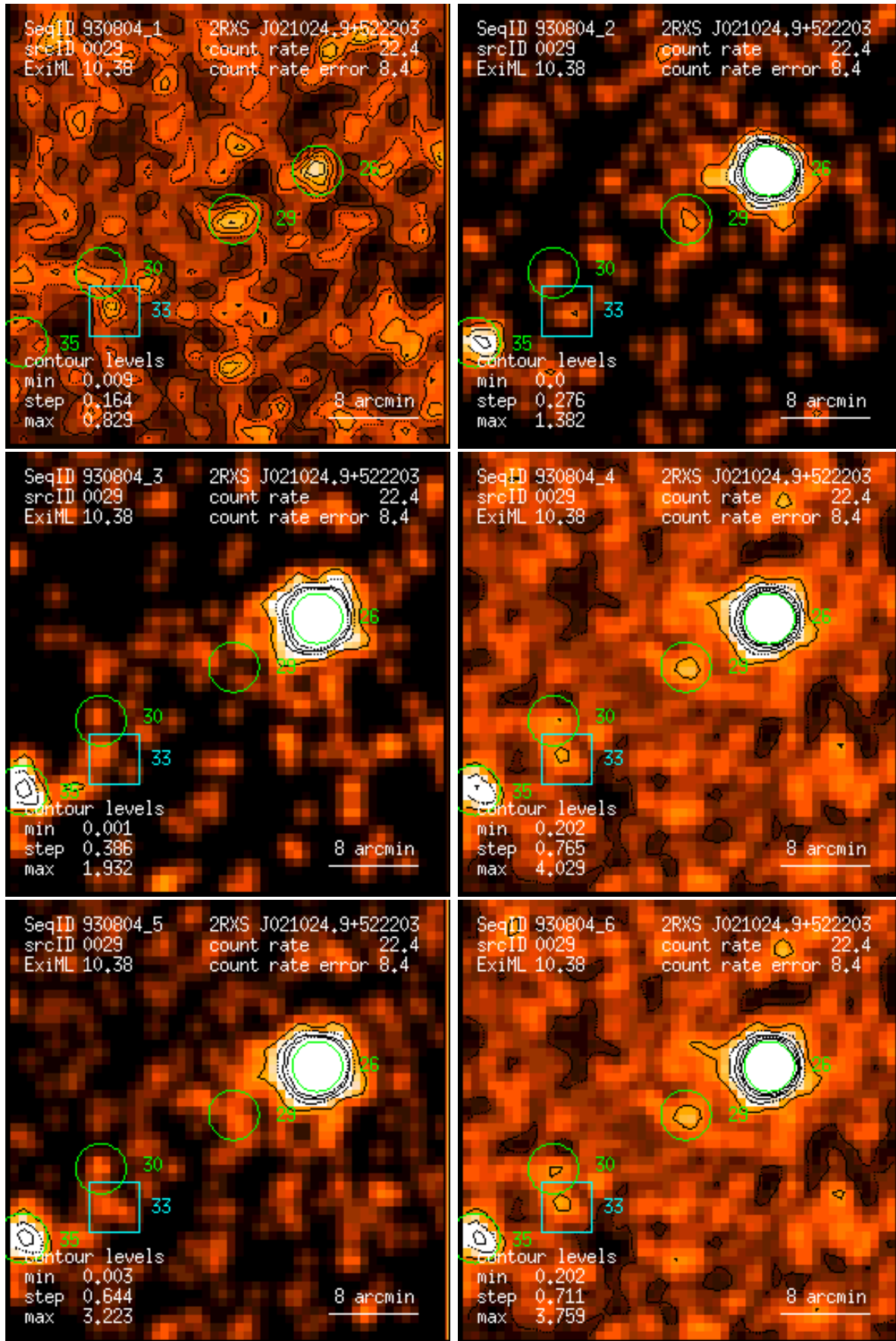
Figure 29: RASS 930804: detection 0029: band rate images, Gaussian filter: (1) PSPC channels 11 – 41, (2) 52 – 90, (3) 91 – 201, (4) 11 – 235, (5) 52 – 201, (6) 11 – 201. Broad band rates in counts/ks. Band rate contour levels in counts/ks/arcmin 2 .
