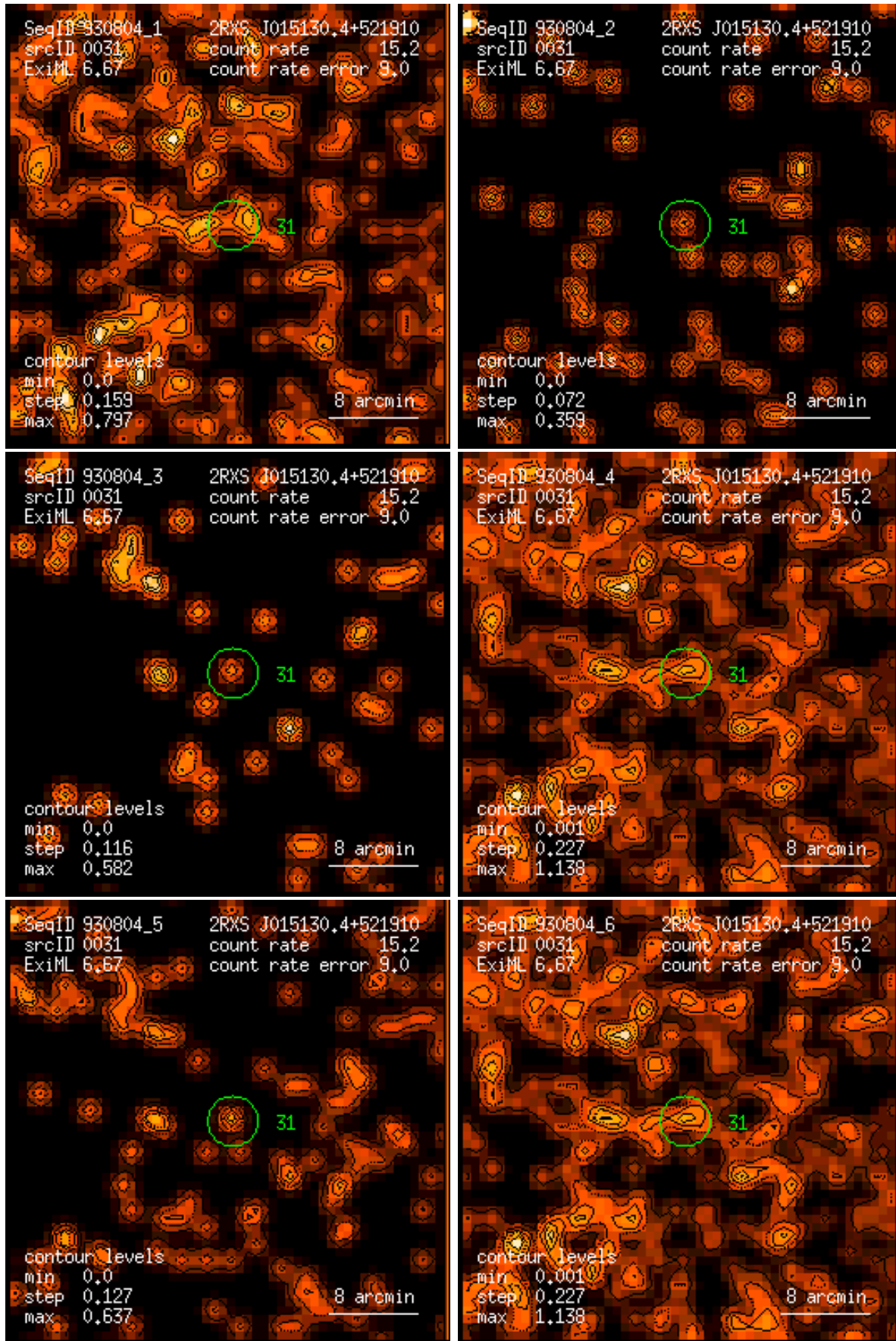
Figure 31: RASS 930804: detection 0031: band rate images, Gaussian filter: (1) PSPC channels 11 – 41, (2) 52 – 90, (3) 91 – 201, (4) 11 – 235, (5) 52 – 201, (6) 11 – 201. Broad band rates in counts/ks. Band rate contour levels in counts/ks/arcmin 2 .
